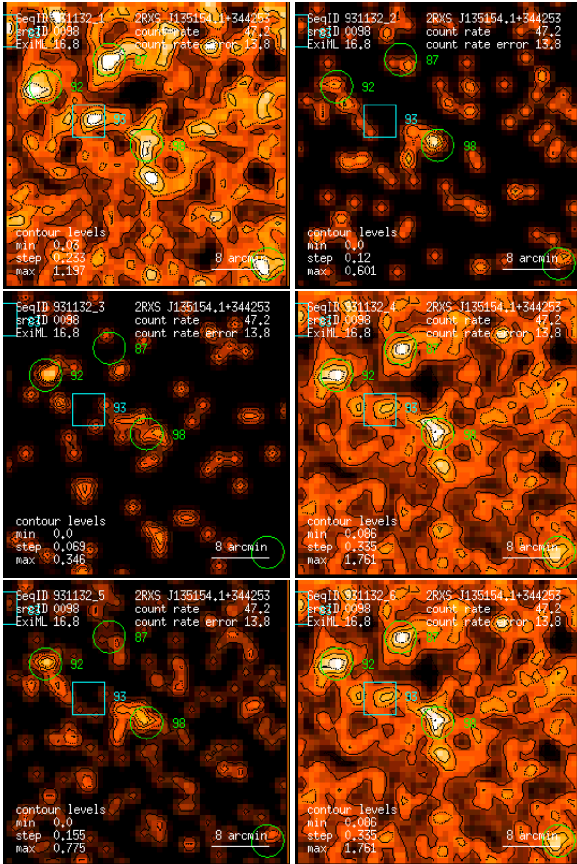
Figure 98: RASS 931132: detection 0098: band rate images, Gaussian filter: (1) PSPC channels 11 – 41, (2) 52 – 90, (3) 91 – 201, (4) 11 – 235, (5) 52 – 201, (6) 11 – 201. Broad band rates in counts/ks. Band rate contour levels in counts/ks/arcmin 2 .
