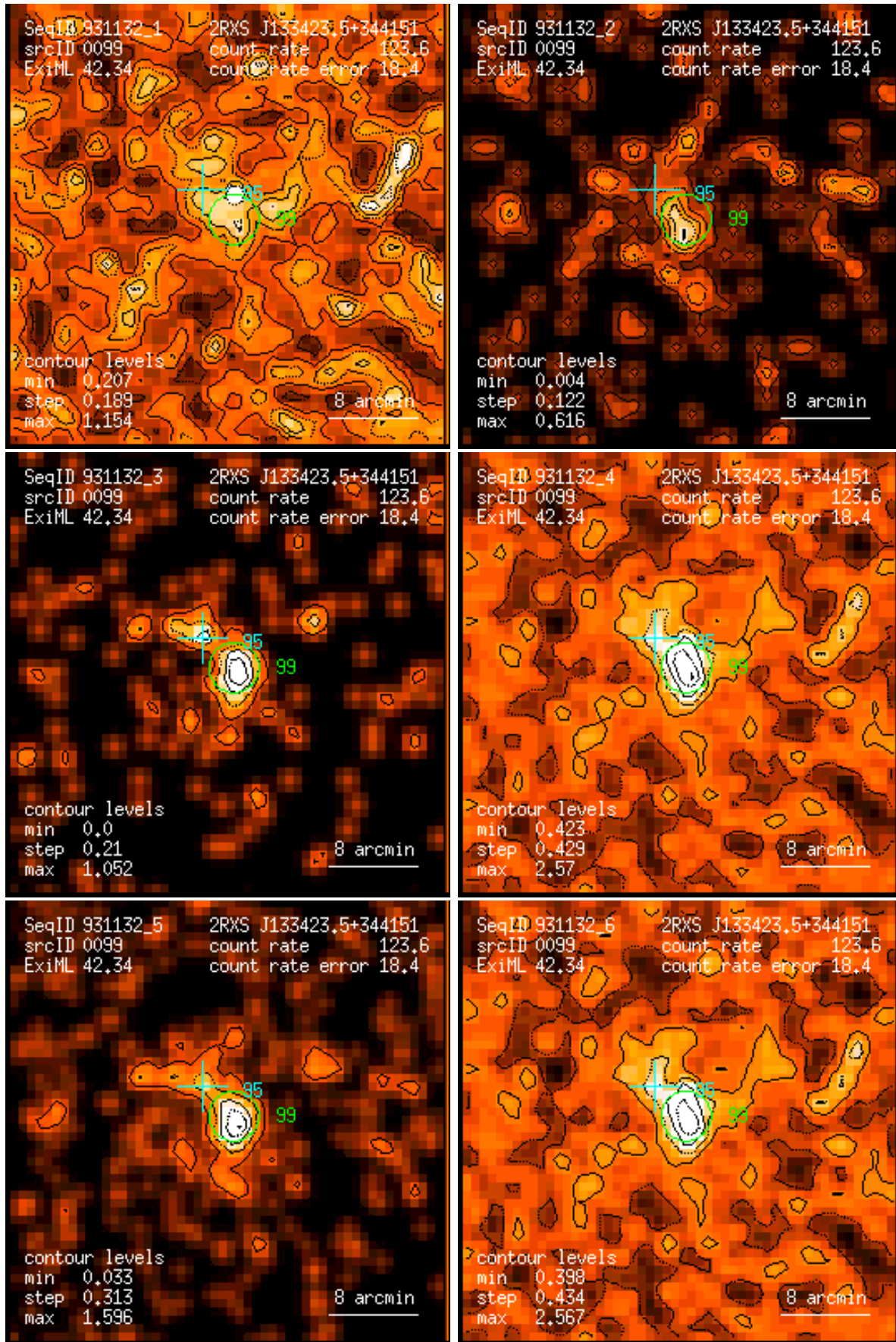
Figure 99: RASS 931132: detection 0099: band rate images, Gaussian filter: (1) PSPC channels 11 – 41, (2) 52 – 90, (3) 91 – 201, (4) 11 – 235, (5) 52 – 201, (6) 11 – 201. Broad band rates in counts/ks. Band rate contour levels in counts/ks/arcmin 2 .
