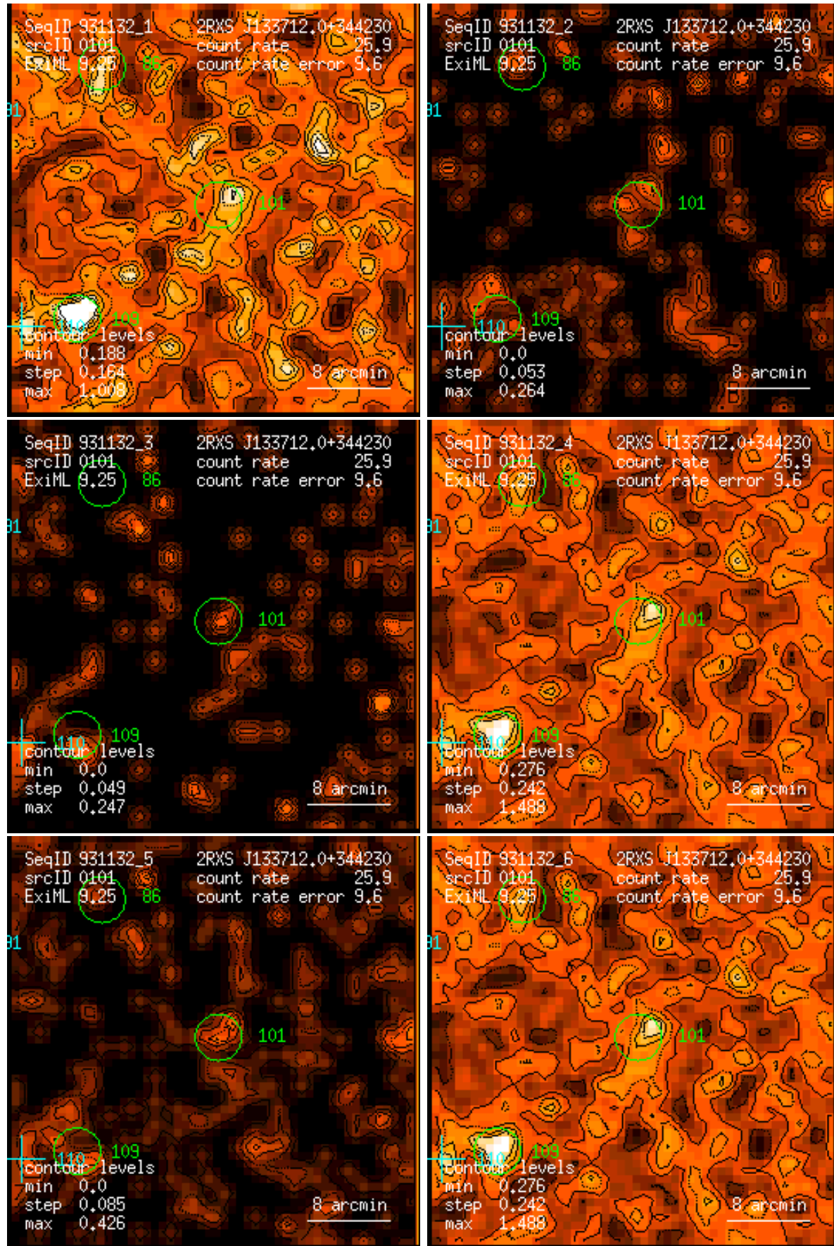
Figure 101: RASS 931132: detection 0101: band rate images, Gaussian filter: (1) PSPC channels 11 – 41, (2) 52 – 90, (3) 91 – 201, (4) 11 – 235, (5) 52 – 201, (6) 11 – 201. Broad band rates in counts/ks. Band rate contour levels in counts/ks/arcmin 2 .
