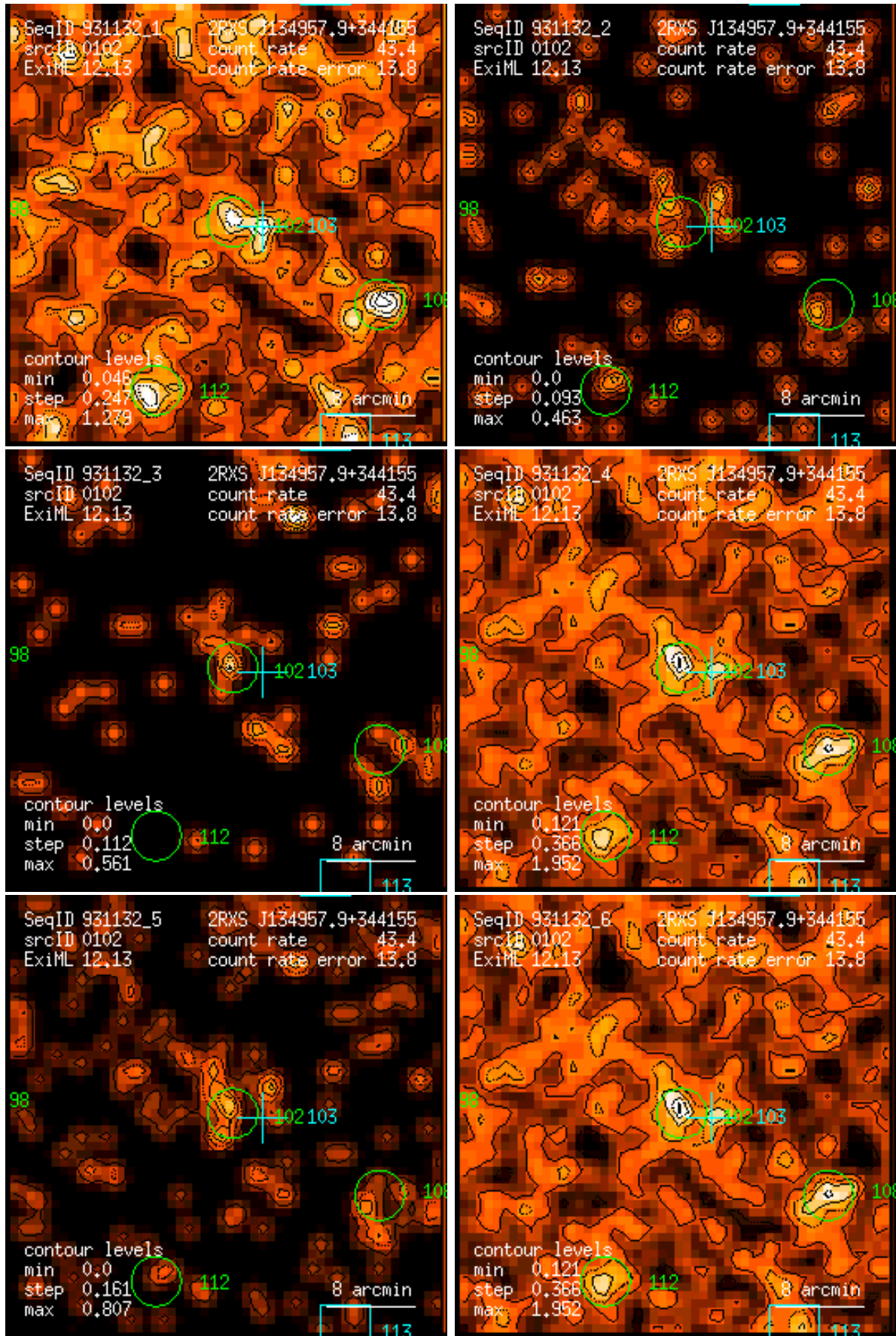
Figure 102: RASS 931132: detection 0102: band rate images, Gaussian filter: (1) PSPC channels 11 – 41, (2) 52 – 90, (3) 91 – 201, (4) 11 – 235, (5) 52 – 201, (6) 11 – 201. Broad band rates in counts/ks. Band rate contour levels in counts/ks/arcmin 2 .
