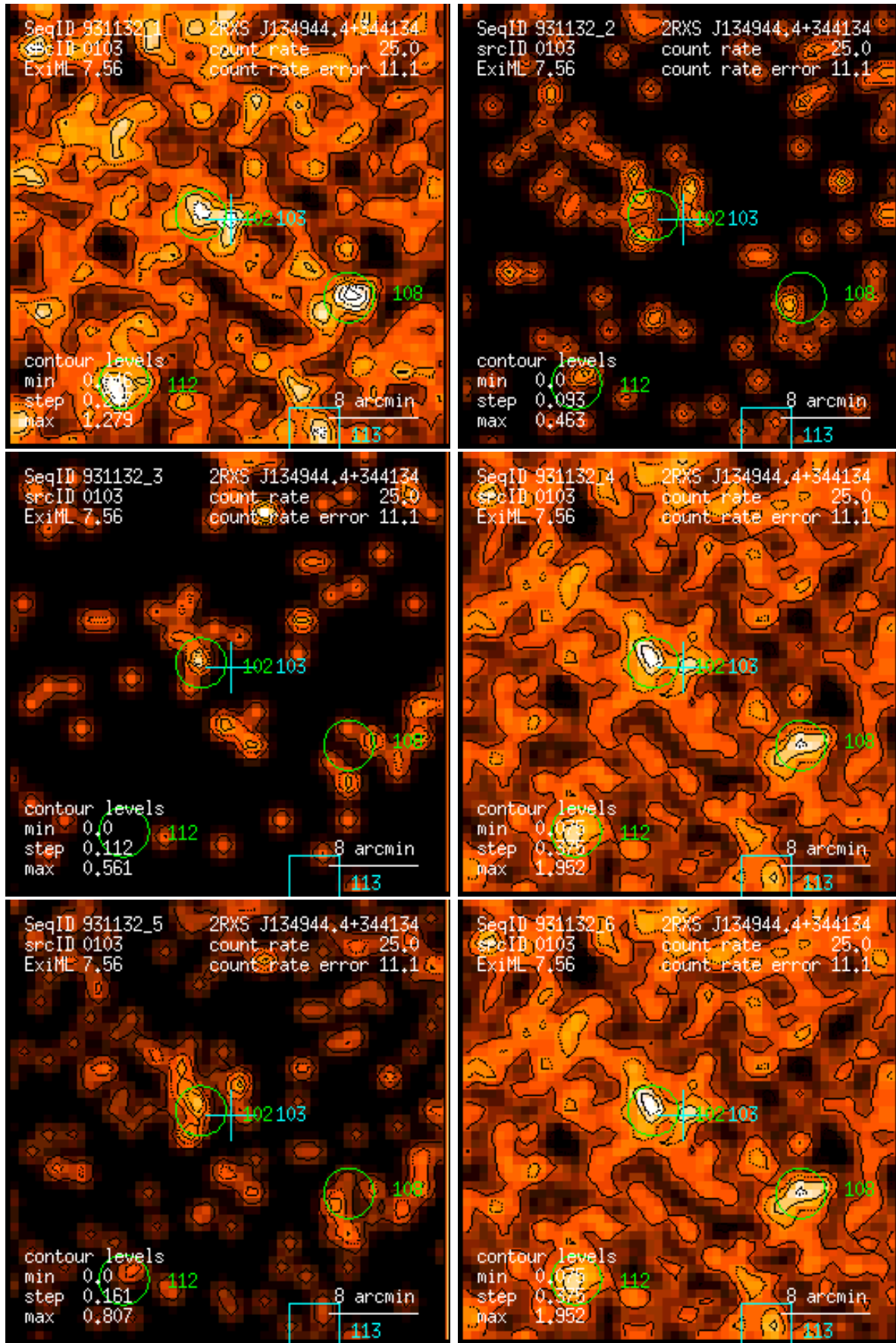
Figure 103: RASS 931132: detection 0103: band rate images, Gaussian filter: (1) PSPC channels 11 – 41, (2) 52 – 90, (3) 91 – 201, (4) 11 – 235, (5) 52 – 201, (6) 11 – 201. Broad band rates in counts/ks. Band rate contour levels in counts/ks/arcmin 2 .
