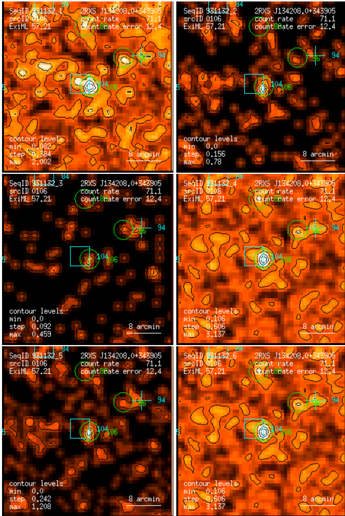
Figure 106: RASS 931132: detection 0106: band rate images, Gaussian filter: (1) PSPC channels 11 – 41, (2) 52 – 90, (3) 91 – 201, (4) 11 – 235, (5) 52 – 201, (6) 11 – 201. Broad band rates in counts/ks. Band rate contour levels in counts/ks/arcmin 2 .
