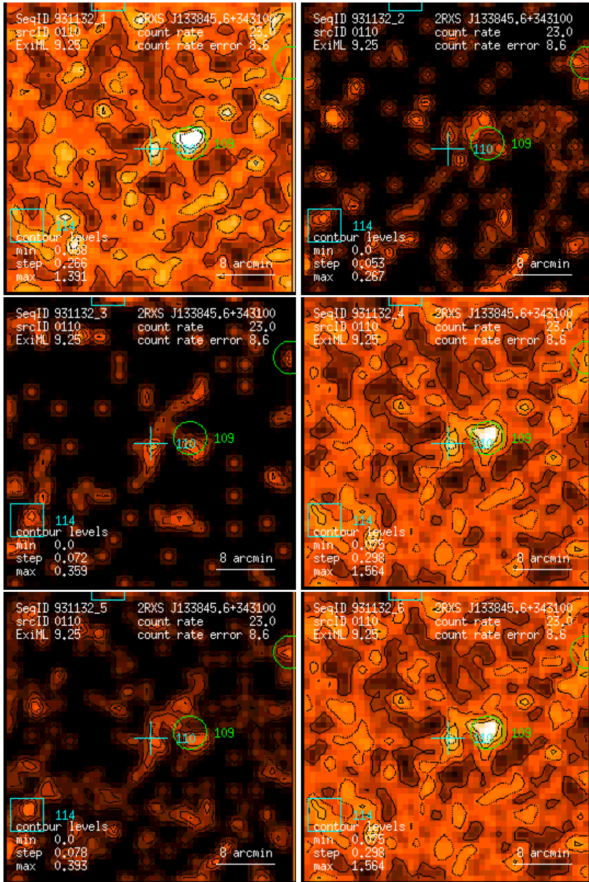
Figure 110: RASS 931132: detection 0110: band rate images, Gaussian filter: (1) PSPC channels 11 – 41, (2) 52 – 90, (3) 91 – 201, (4) 11 – 235, (5) 52 – 201, (6) 11 – 201. Broad band rates in counts/ks. Band rate contour levels in counts/ks/arcmin 2 .
