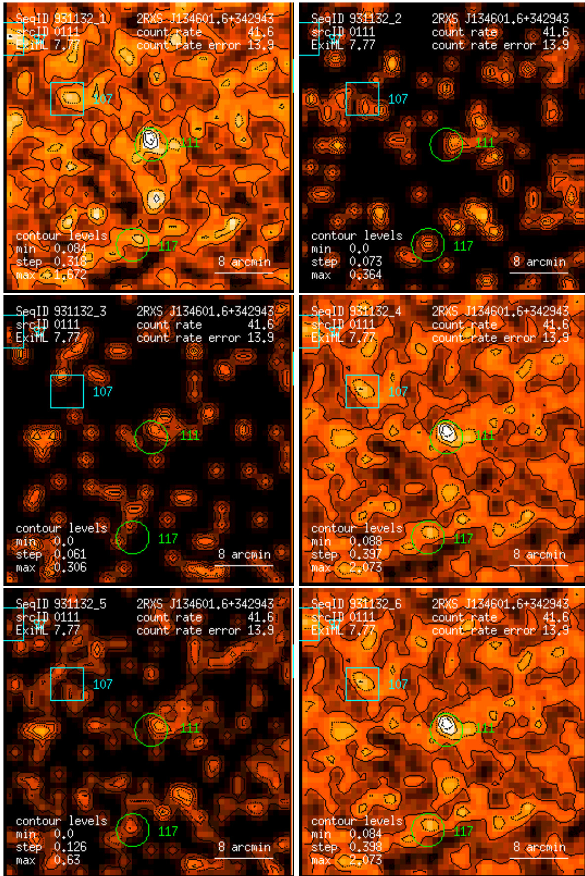
Figure 111: RASS 931132: detection 0111: band rate images, Gaussian filter: (1) PSPC channels 11 – 41, (2) 52 – 90, (3) 91 – 201, (4) 11 – 235, (5) 52 – 201, (6) 11 – 201. Broad band rates in counts/ks. Band rate contour levels in counts/ks/arcmin 2 .
