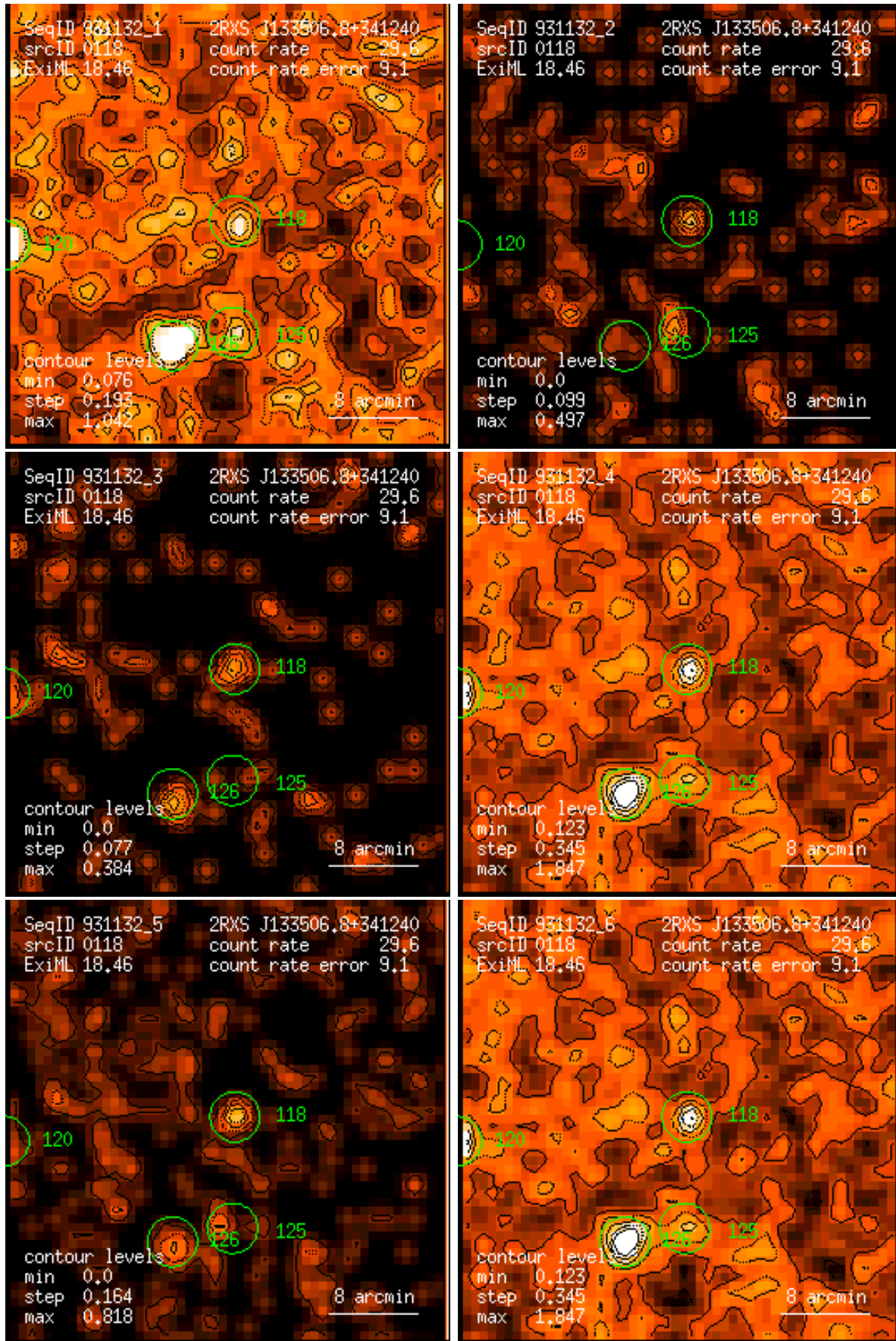
Figure 118: RASS 931132: detection 0118: band rate images, Gaussian filter: (1) PSPC channels 11 – 41, (2) 52 – 90, (3) 91 – 201, (4) 11 – 235, (5) 52 – 201, (6) 11 – 201. Broad band rates in counts/ks. Band rate contour levels in counts/ks/arcmin 2 .
