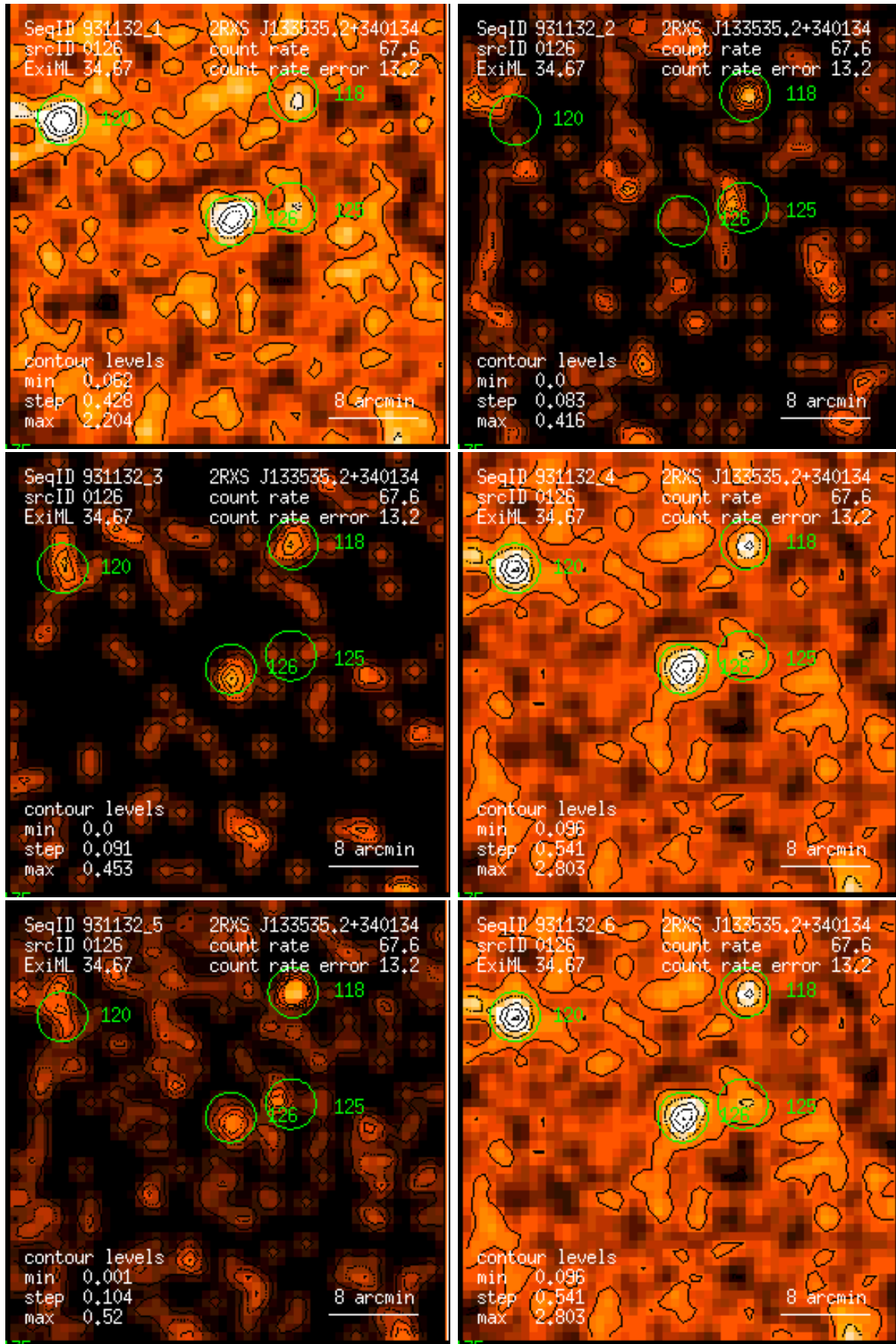
Figure 126: RASS 931132: detection 0126: band rate images, Gaussian filter: (1) PSPC channels 11 – 41, (2) 52 – 90, (3) 91 – 201, (4) 11 – 235, (5) 52 – 201, (6) 11 – 201. Broad band rates in counts/ks. Band rate contour levels in counts/ks/arcmin 2 .
