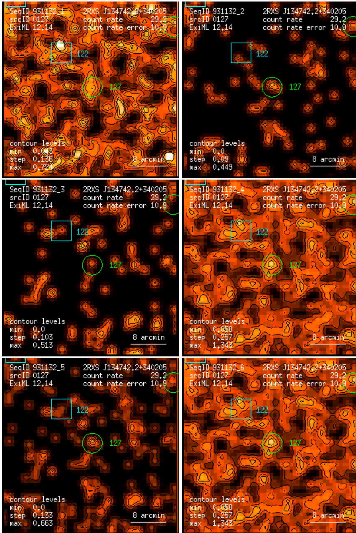
Figure 127: RASS 931132: detection 0127: band rate images, Gaussian filter: (1) PSPC channels 11 – 41, (2) 52 – 90, (3) 91 – 201, (4) 11 – 235, (5) 52 – 201, (6) 11 – 201. Broad band rates in counts/ks. Band rate contour levels in counts/ks/arcmin 2 .
