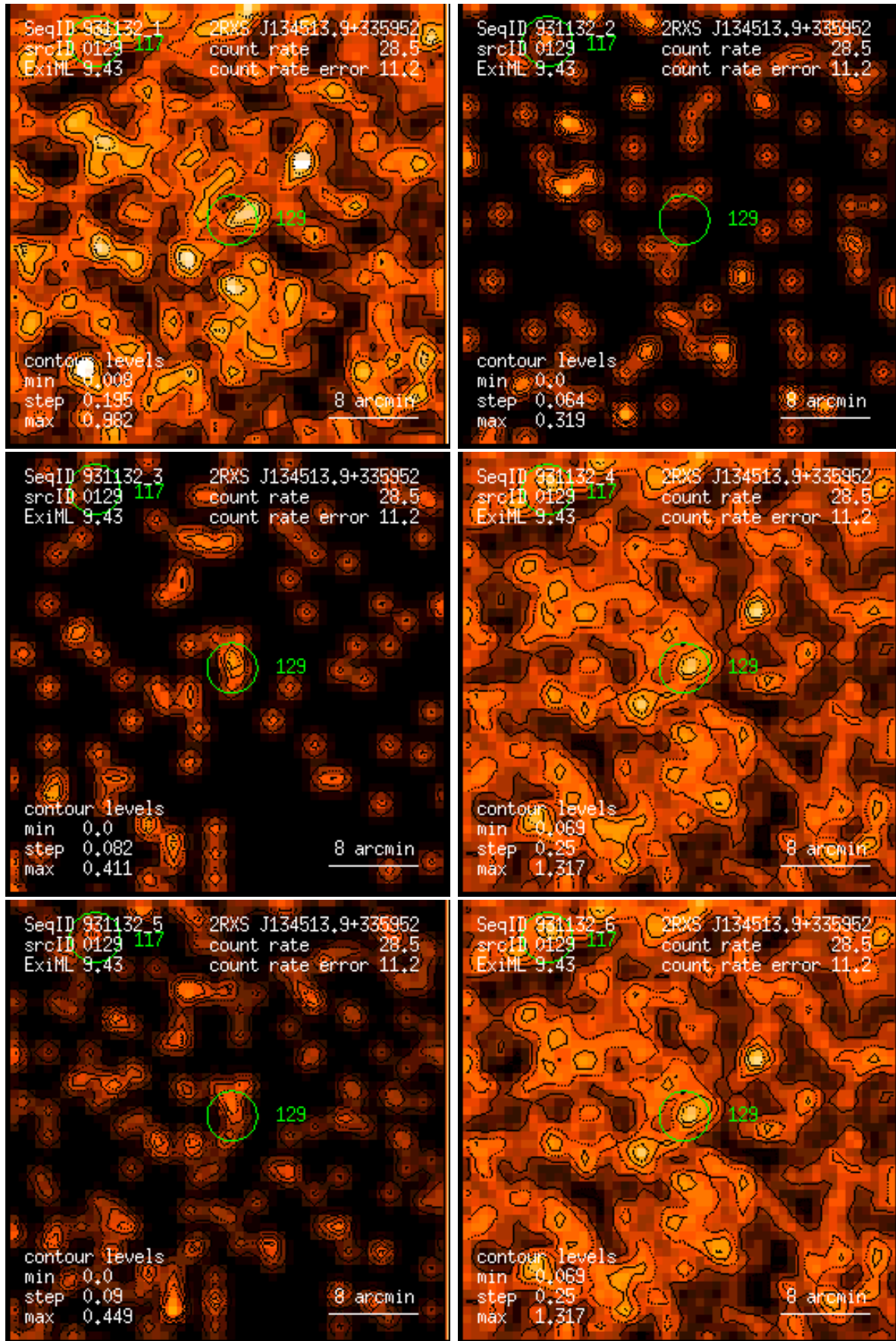
Figure 129: RASS 931132: detection 0129: band rate images, Gaussian filter: (1) PSPC channels 11 – 41, (2) 52 – 90, (3) 91 – 201, (4) 11 – 235, (5) 52 – 201, (6) 11 – 201. Broad band rates in counts/ks. Band rate contour levels in counts/ks/arcmin 2 .
