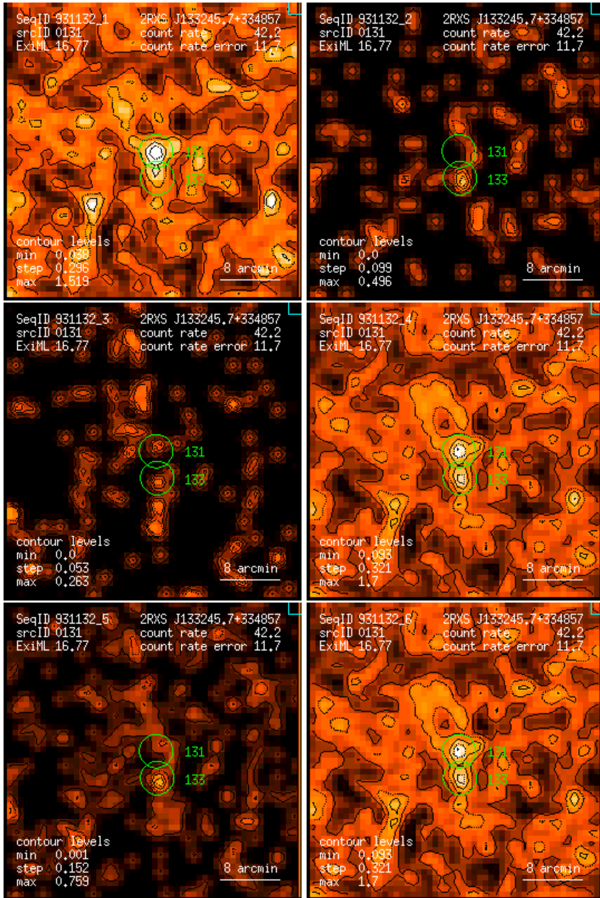
Figure 131: RASS 931132: detection 0131: band rate images, Gaussian filter: (1) PSPC channels 11 – 41, (2) 52 – 90, (3) 91 – 201, (4) 11 – 235, (5) 52 – 201, (6) 11 – 201. Broad band rates in counts/ks. Band rate contour levels in counts/ks/arcmin 2 .
