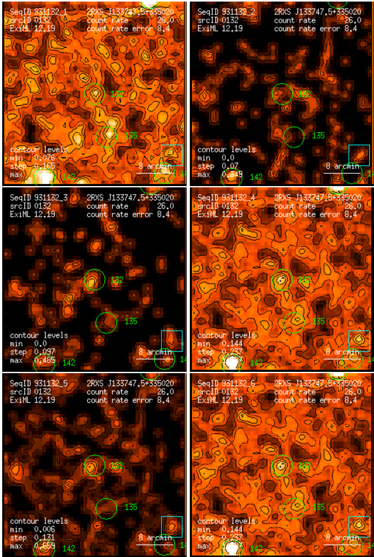
Figure 132: RASS 931132: detection 0132: band rate images, Gaussian filter: (1) PSPC channels 11 – 41, (2) 52 – 90, (3) 91 – 201, (4) 11 – 235, (5) 52 – 201, (6) 11 – 201. Broad band rates in counts/ks. Band rate contour levels in counts/ks/arcmin 2 .
