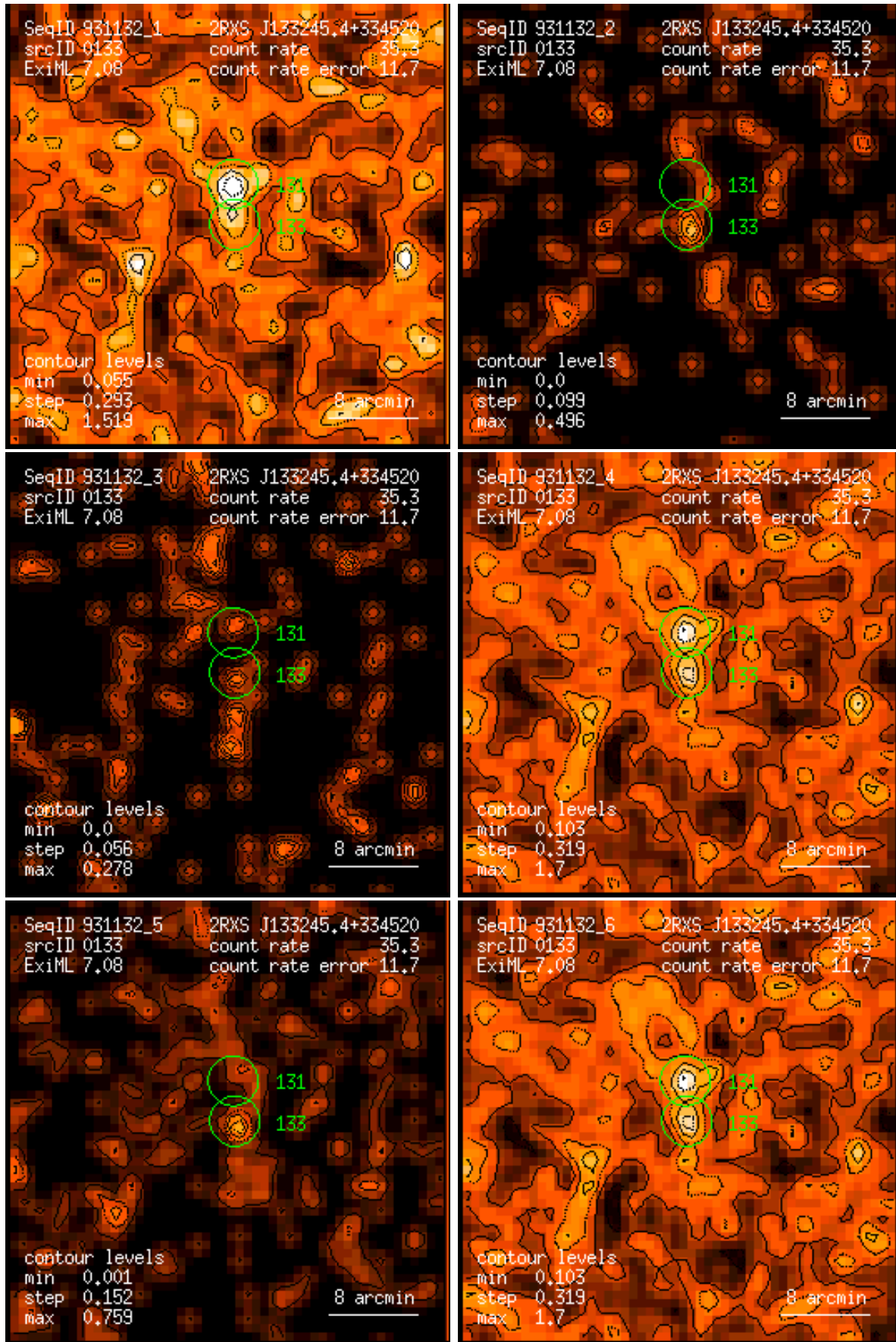
Figure 133: RASS 931132: detection 0133: band rate images, Gaussian filter: (1) PSPC channels 11 – 41, (2) 52 – 90, (3) 91 – 201, (4) 11 – 235, (5) 52 – 201, (6) 11 – 201. Broad band rates in counts/ks. Band rate contour levels in counts/ks/arcmin 2 .
