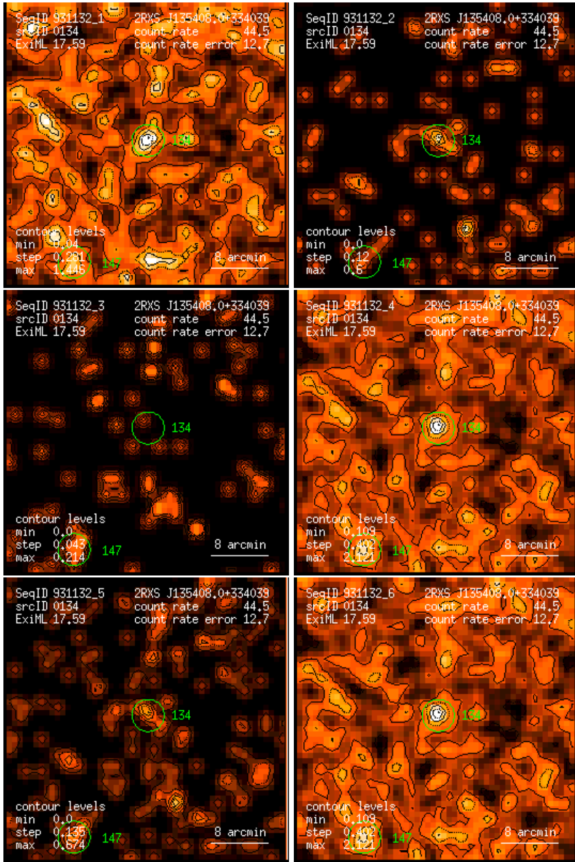
Figure 134: RASS 931132: detection 0134: band rate images, Gaussian filter: (1) PSPC channels 11 – 41, (2) 52 – 90, (3) 91 – 201, (4) 11 – 235, (5) 52 – 201, (6) 11 – 201. Broad band rates in counts/ks. Band rate contour levels in counts/ks/arcmin 2 .
