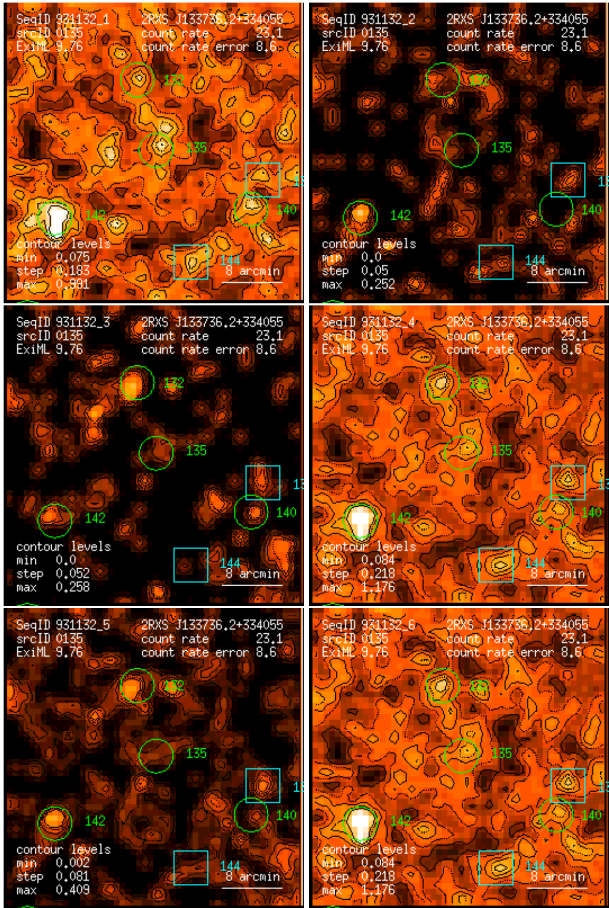
Figure 135: RASS 931132: detection 0135: band rate images, Gaussian filter: (1) PSPC channels 11 – 41, (2) 52 – 90, (3) 91 – 201, (4) 11 – 235, (5) 52 – 201, (6) 11 – 201. Broad band rates in counts/ks. Band rate contour levels in counts/ks/arcmin 2 .
