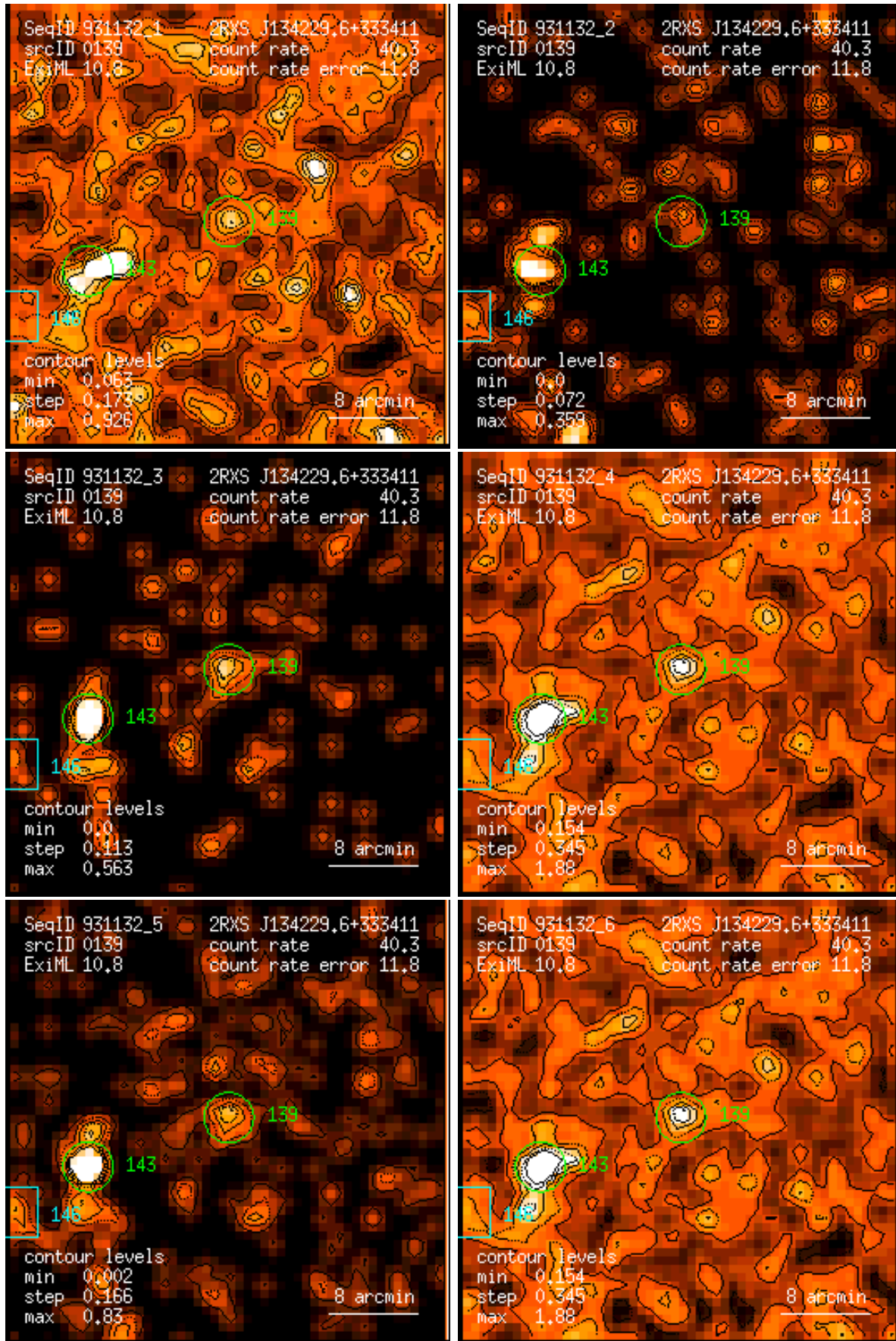
Figure 139: RASS 931132: detection 0139: band rate images, Gaussian filter: (1) PSPC channels 11 – 41, (2) 52 – 90, (3) 91 – 201, (4) 11 – 235, (5) 52 – 201, (6) 11 – 201. Broad band rates in counts/ks. Band rate contour levels in counts/ks/arcmin 2 .
