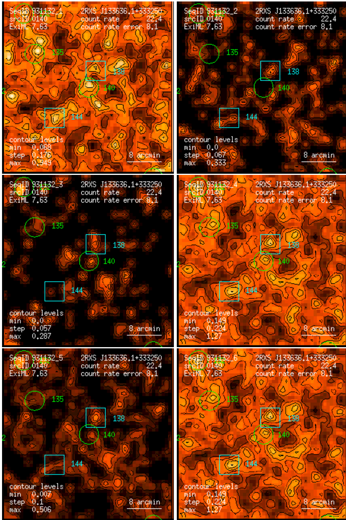
Figure 140: RASS 931132: detection 0140: band rate images, Gaussian filter: (1) PSPC channels 11 – 41, (2) 52 – 90, (3) 91 – 201, (4) 11 – 235, (5) 52 – 201, (6) 11 – 201. Broad band rates in counts/ks. Band rate contour levels in counts/ks/arcmin 2 .
