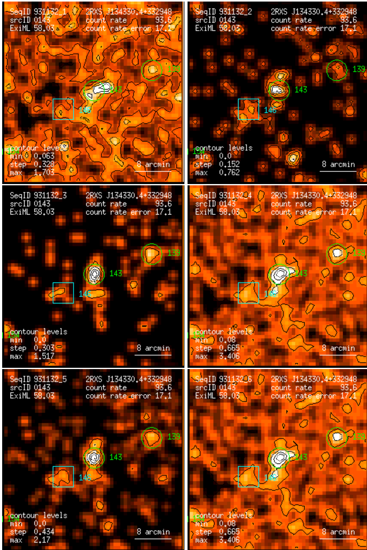
Figure 143: RASS 931132: detection 0143: band rate images, Gaussian filter: (1) PSPC channels 11 – 41, (2) 52 – 90, (3) 91 – 201, (4) 11 – 235, (5) 52 – 201, (6) 11 – 201. Broad band rates in counts/ks. Band rate contour levels in counts/ks/arcmin 2 .
