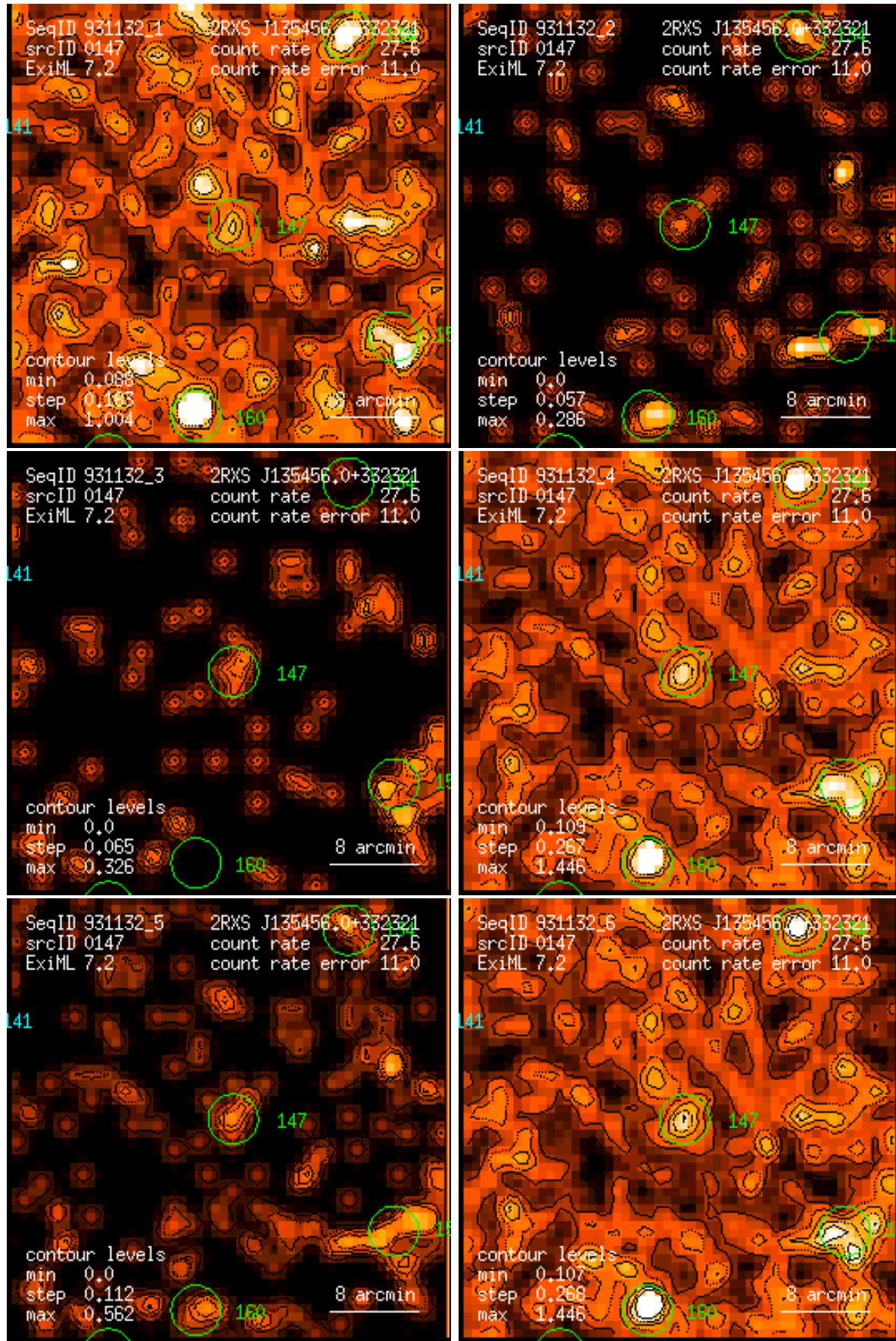
Figure 147: RASS 931132: detection 0147: band rate images, Gaussian filter: (1) PSPC channels 11 – 41, (2) 52 – 90, (3) 91 – 201, (4) 11 – 235, (5) 52 – 201, (6) 11 – 201. Broad band rates in counts/ks. Band rate contour levels in counts/ks/arcmin 2 .
