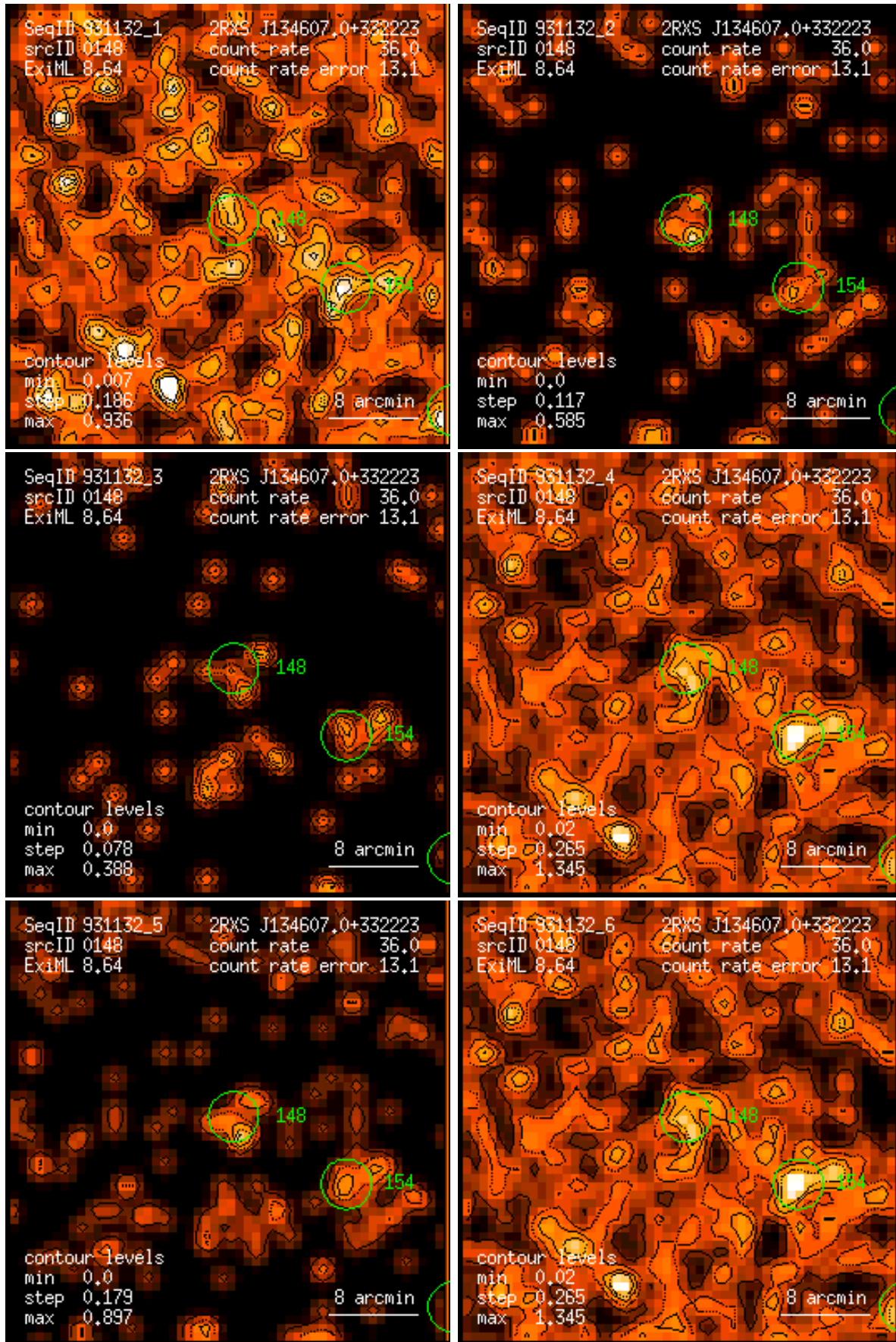
Figure 148: RASS 931132: detection 0148: band rate images, Gaussian filter: (1) PSPC channels 11 – 41, (2) 52 – 90, (3) 91 – 201, (4) 11 – 235, (5) 52 – 201, (6) 11 – 201. Broad band rates in counts/ks. Band rate contour levels in counts/ks/arcmin 2 .
