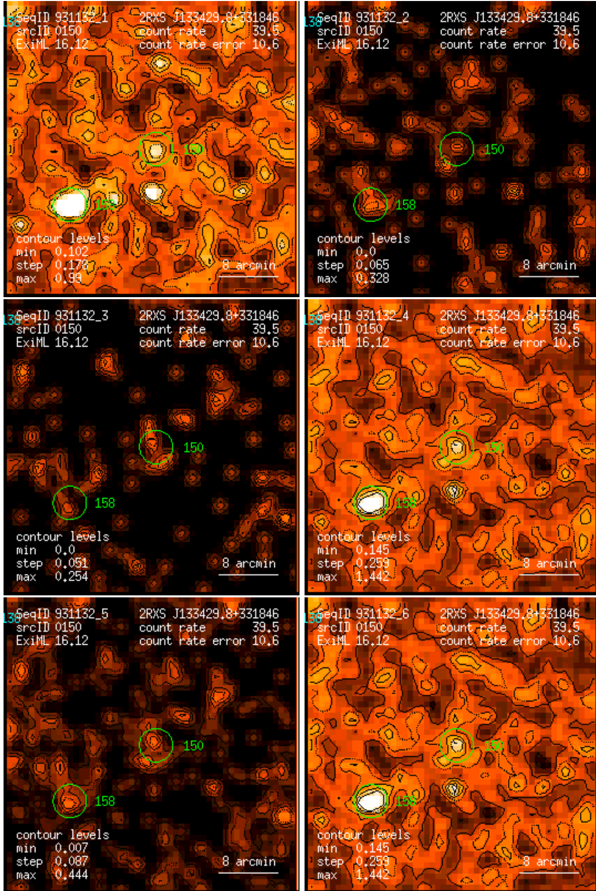
Figure 150: RASS 931132: detection 0150: band rate images, Gaussian filter: (1) PSPC channels 11 – 41, (2) 52 – 90, (3) 91 – 201, (4) 11 – 235, (5) 52 – 201, (6) 11 – 201. Broad band rates in counts/ks. Band rate contour levels in counts/ks/arcmin 2 .
