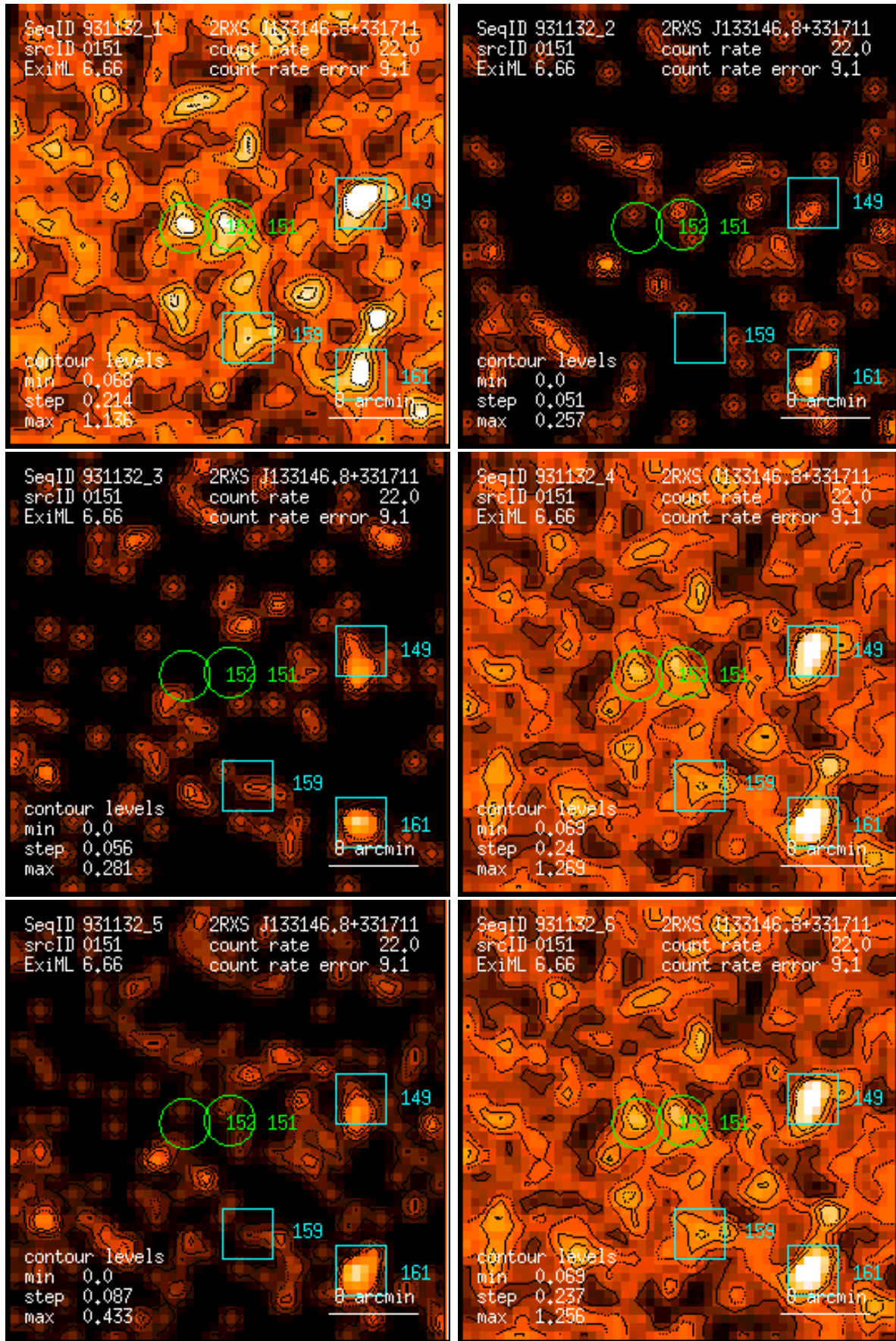
Figure 151: RASS 931132: detection 0151: band rate images, Gaussian filter: (1) PSPC channels 11 – 41, (2) 52 – 90, (3) 91 – 201, (4) 11 – 235, (5) 52 – 201, (6) 11 – 201. Broad band rates in counts/ks. Band rate contour levels in counts/ks/arcmin 2 .
