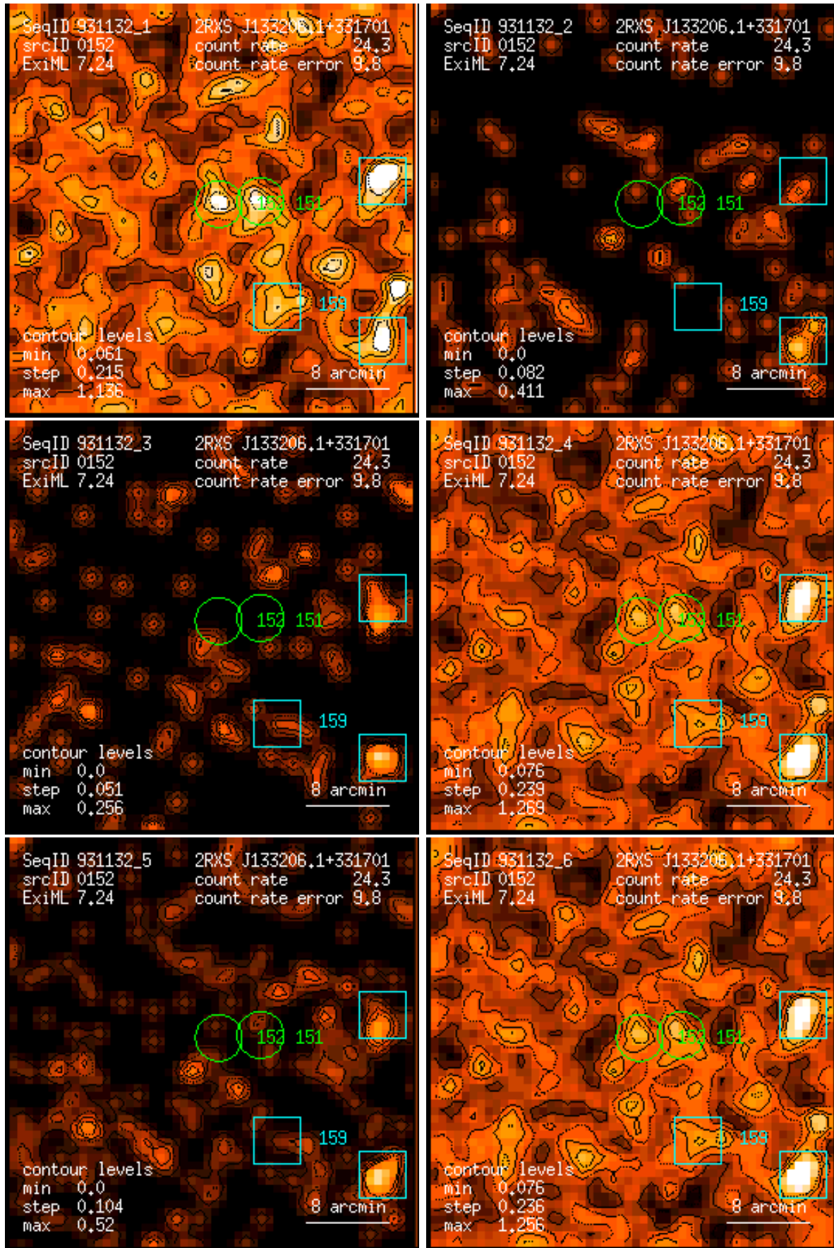
Figure 152: RASS 931132: detection 0152: band rate images, Gaussian filter: (1) PSPC channels 11 – 41, (2) 52 – 90, (3) 91 – 201, (4) 11 – 235, (5) 52 – 201, (6) 11 – 201. Broad band rates in counts/ks. Band rate contour levels in counts/ks/arcmin 2 .
