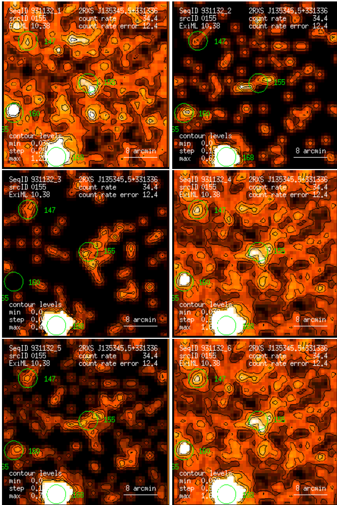
Figure 155: RASS 931132: detection 0155: band rate images, Gaussian filter: (1) PSPC channels 11 – 41, (2) 52 – 90, (3) 91 – 201, (4) 11 – 235, (5) 52 – 201, (6) 11 – 201. Broad band rates in counts/ks. Band rate contour levels in counts/ks/arcmin 2 .
