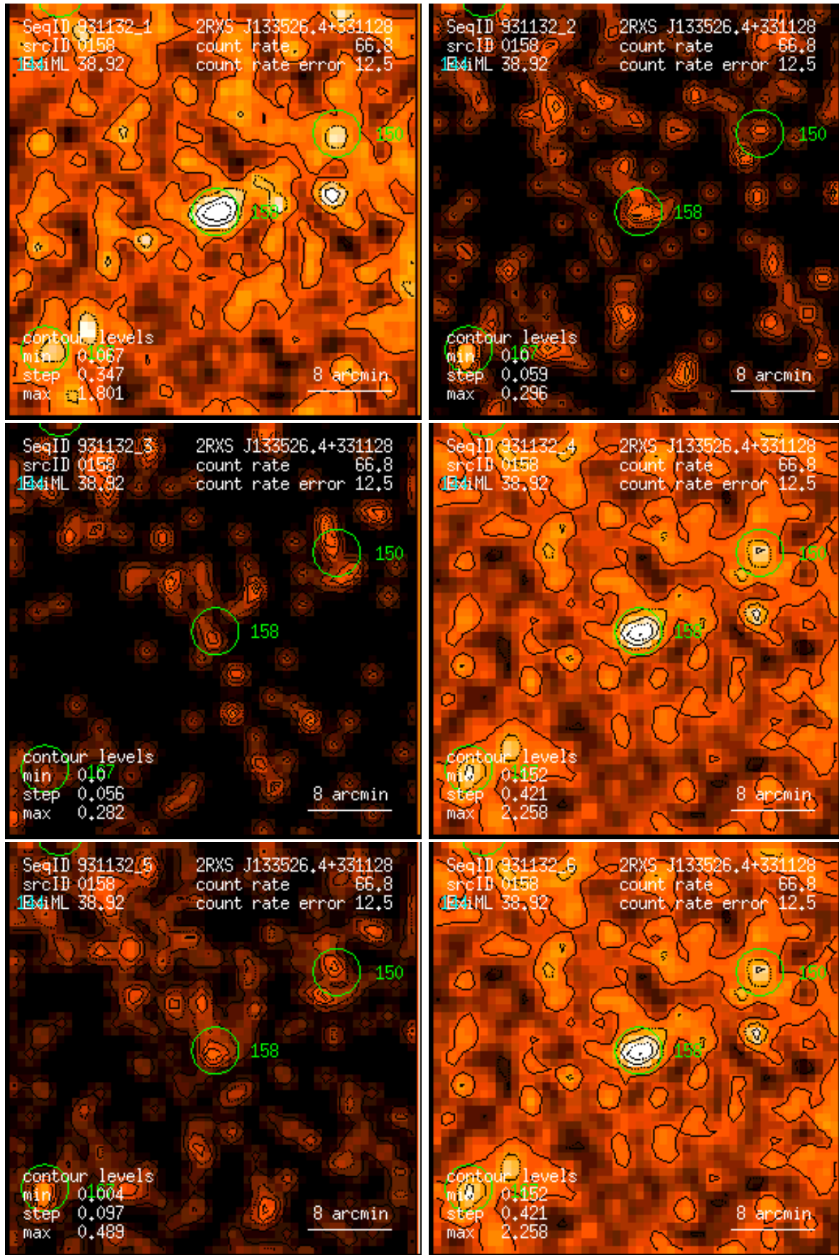
Figure 158: RASS 931132: detection 0158: band rate images, Gaussian filter: (1) PSPC channels 11 – 41, (2) 52 – 90, (3) 91 – 201, (4) 11 – 235, (5) 52 – 201, (6) 11 – 201. Broad band rates in counts/ks. Band rate contour levels in counts/ks/arcmin 2 .
