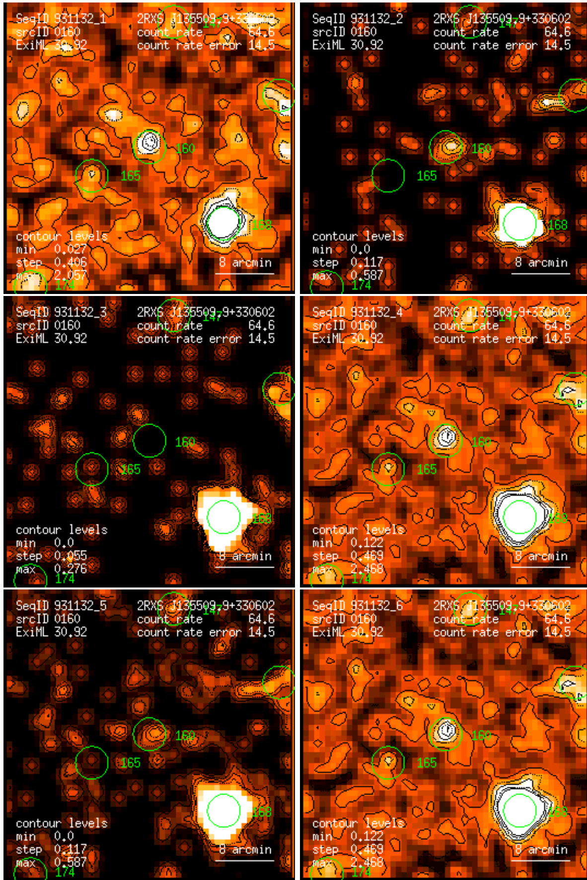
Figure 160: RASS 931132: detection 0160: band rate images, Gaussian filter: (1) PSPC channels 11 – 41, (2) 52 – 90, (3) 91 – 201, (4) 11 – 235, (5) 52 – 201, (6) 11 – 201. Broad band rates in counts/ks. Band rate contour levels in counts/ks/arcmin 2 .
