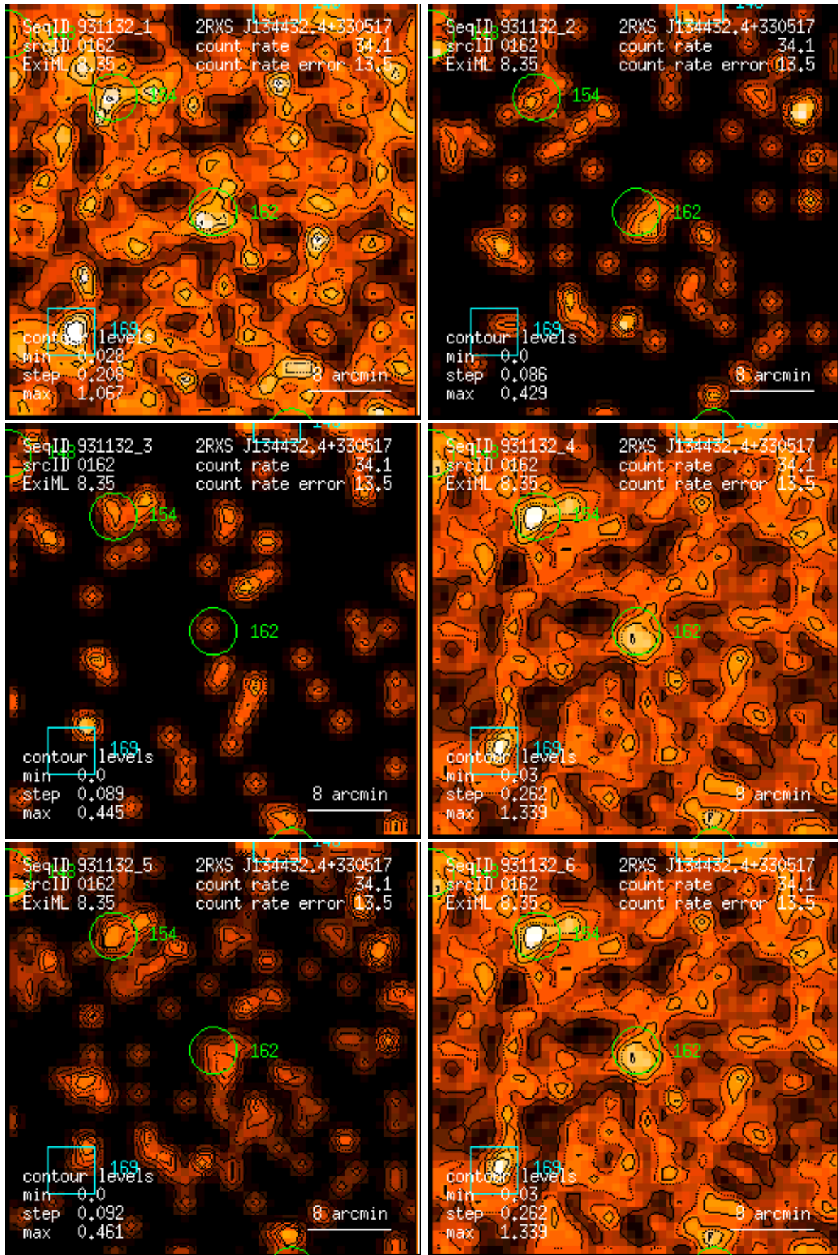
Figure 162: RASS 931132: detection 0162: band rate images, Gaussian filter: (1) PSPC channels 11 – 41, (2) 52 – 90, (3) 91 – 201, (4) 11 – 235, (5) 52 – 201, (6) 11 – 201. Broad band rates in counts/ks. Band rate contour levels in counts/ks/arcmin 2 .
