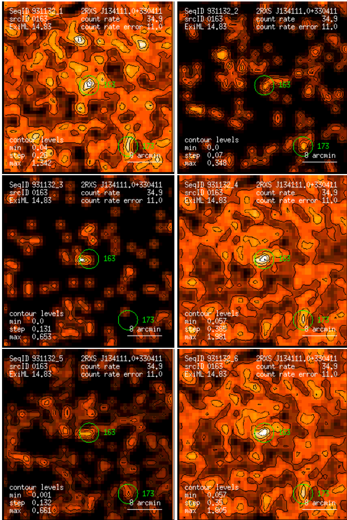
Figure 163: RASS 931132: detection 0163: band rate images, Gaussian filter: (1) PSPC channels 11 – 41, (2) 52 – 90, (3) 91 – 201, (4) 11 – 235, (5) 52 – 201, (6) 11 – 201. Broad band rates in counts/ks. Band rate contour levels in counts/ks/arcmin 2 .
