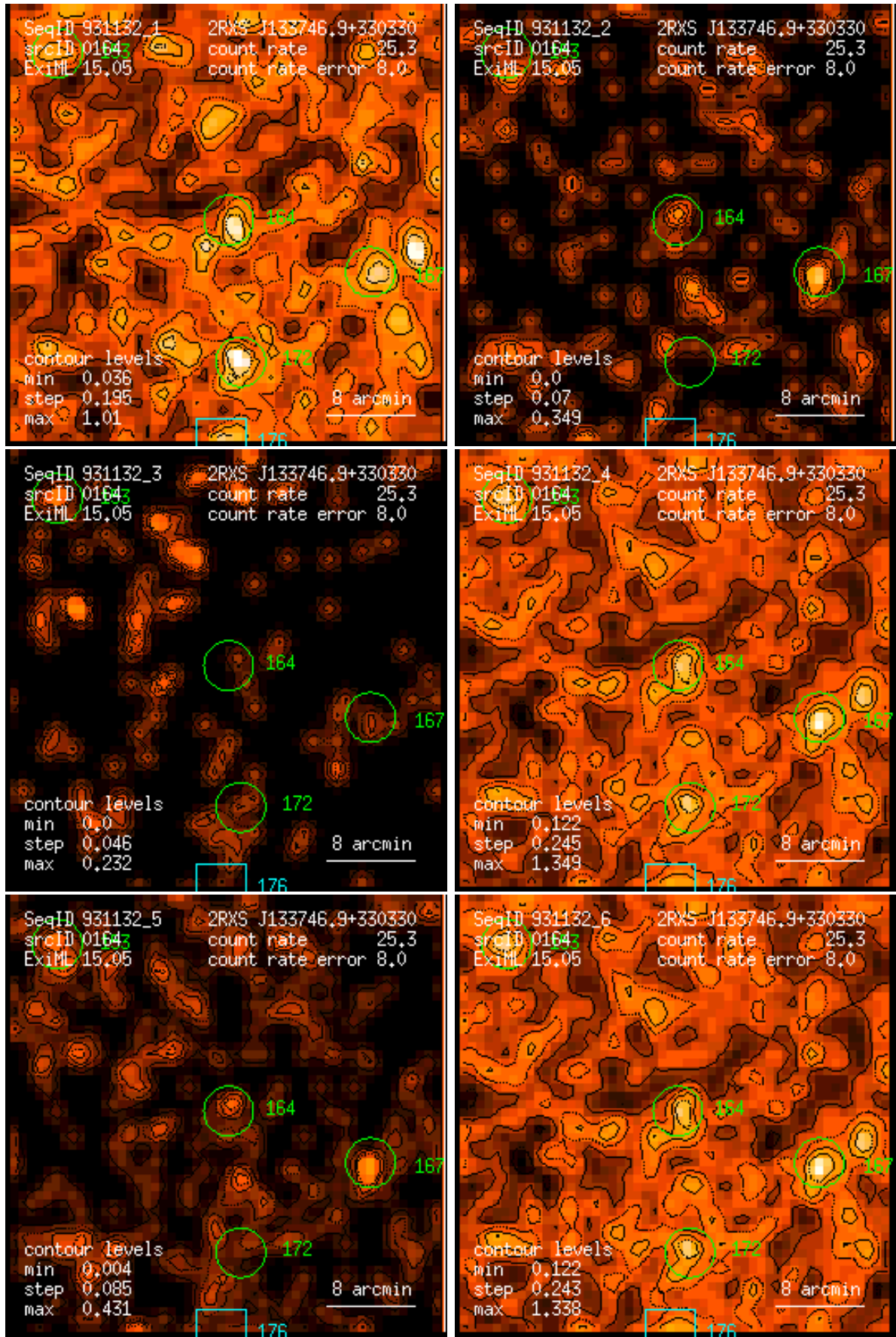
Figure 164: RASS 931132: detection 0164: band rate images, Gaussian filter: (1) PSPC channels 11 – 41, (2) 52 – 90, (3) 91 – 201, (4) 11 – 235, (5) 52 – 201, (6) 11 – 201. Broad band rates in counts/ks. Band rate contour levels in counts/ks/arcmin 2 .
