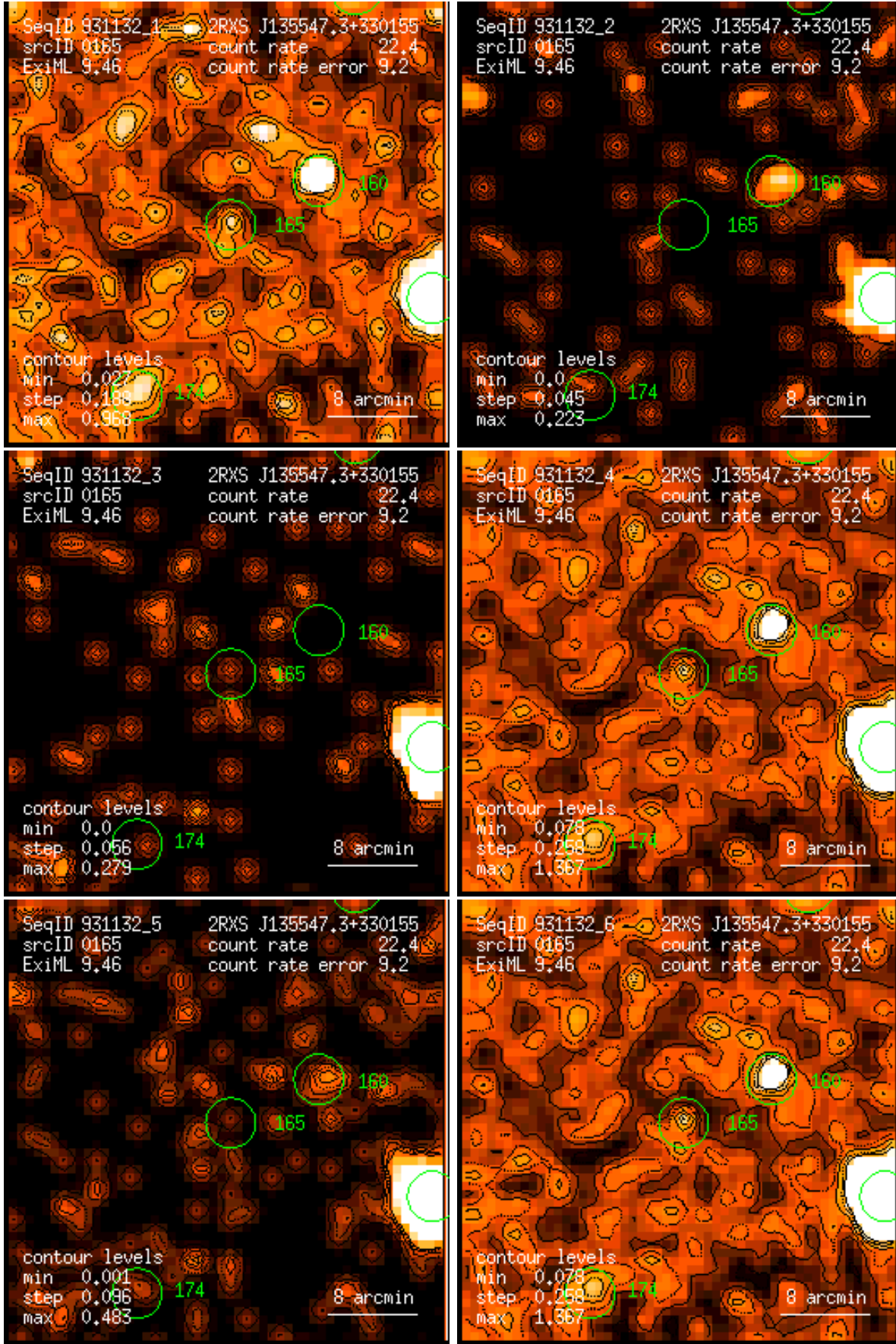
Figure 165: RASS 931132: detection 0165: band rate images, Gaussian filter: (1) PSPC channels 11 – 41, (2) 52 – 90, (3) 91 – 201, (4) 11 – 235, (5) 52 – 201, (6) 11 – 201. Broad band rates in counts/ks. Band rate contour levels in counts/ks/arcmin 2 .
