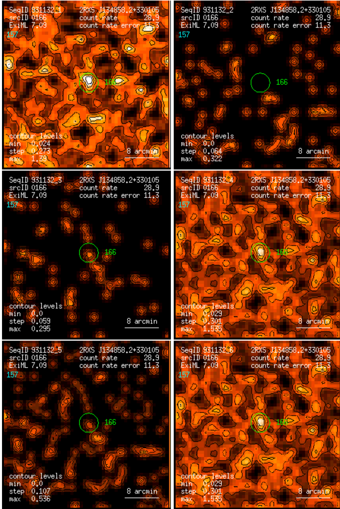
Figure 166: RASS 931132: detection 0166: band rate images, Gaussian filter: (1) PSPC channels 11 – 41, (2) 52 – 90, (3) 91 – 201, (4) 11 – 235, (5) 52 – 201, (6) 11 – 201. Broad band rates in counts/ks. Band rate contour levels in counts/ks/arcmin 2 .
