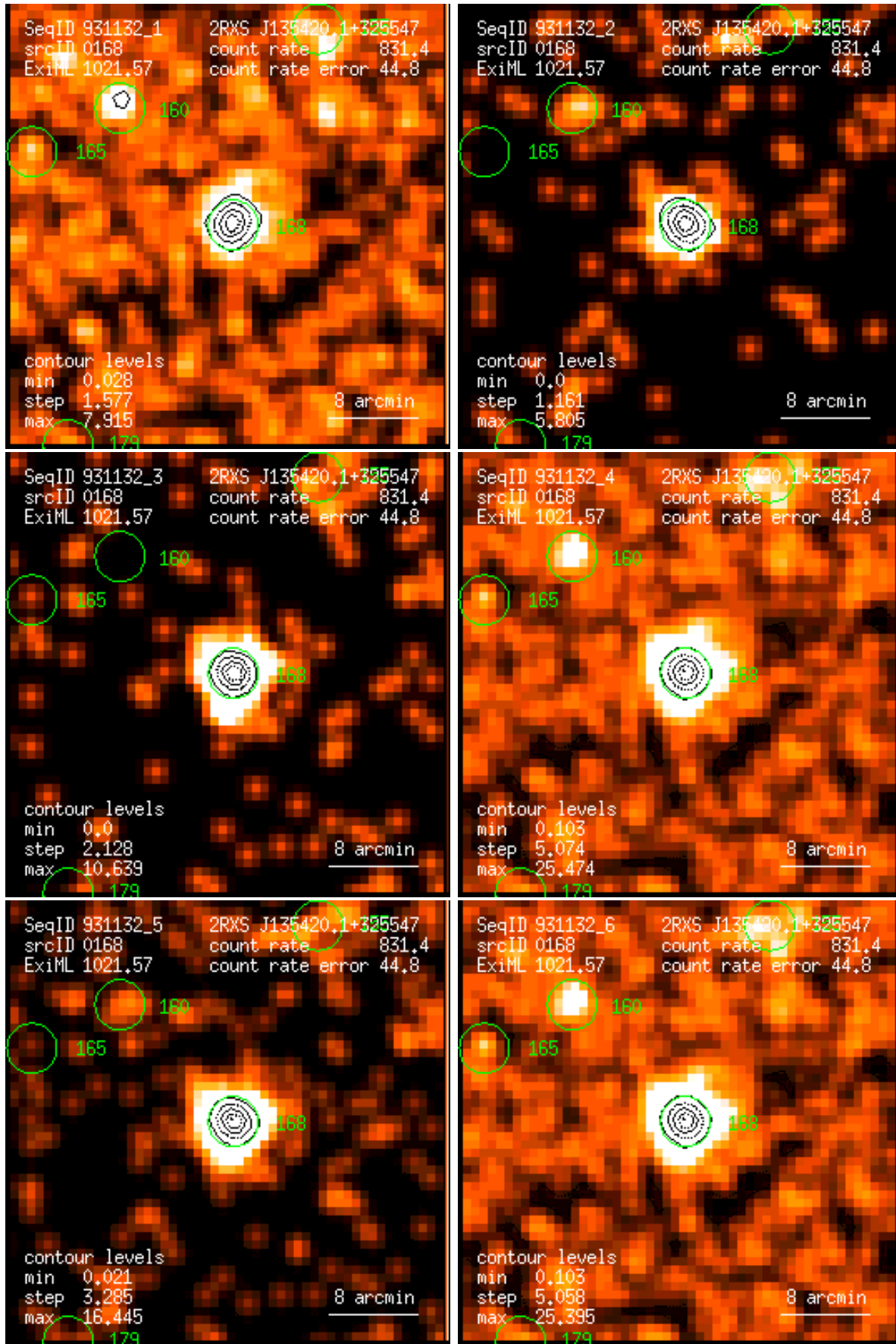
Figure 168: RASS 931132: detection 0168: band rate images, Gaussian filter: (1) PSPC channels 11 – 41, (2) 52 – 90, (3) 91 – 201, (4) 11 – 235, (5) 52 – 201, (6) 11 – 201. Broad band rates in counts/ks. Band rate contour levels in counts/ks/arcmin 2 .
