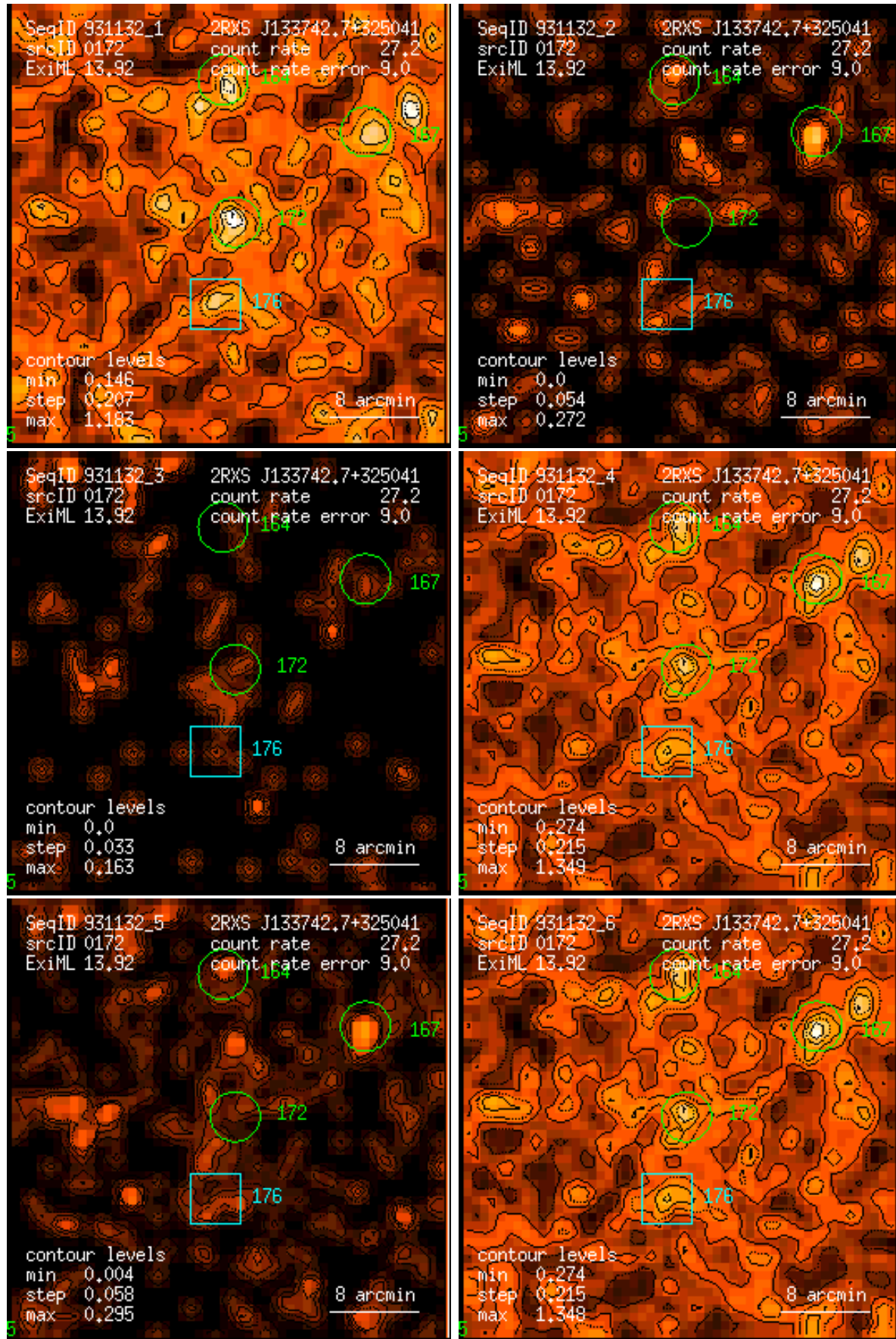
Figure 172: RASS 931132: detection 0172: band rate images, Gaussian filter: (1) PSPC channels 11 – 41, (2) 52 – 90, (3) 91 – 201, (4) 11 – 235, (5) 52 – 201, (6) 11 – 201. Broad band rates in counts/ks. Band rate contour levels in counts/ks/arcmin 2 .
