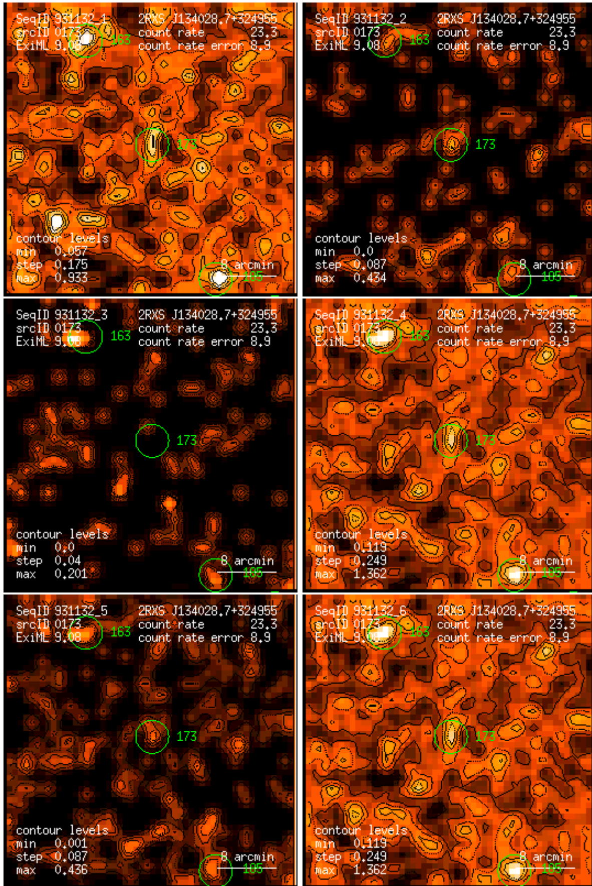
Figure 173: RASS 931132: detection 0173: band rate images, Gaussian filter: (1) PSPC channels 11 – 41, (2) 52 – 90, (3) 91 – 201, (4) 11 – 235, (5) 52 – 201, (6) 11 – 201. Broad band rates in counts/ks. Band rate contour levels in counts/ks/arcmin 2 .
