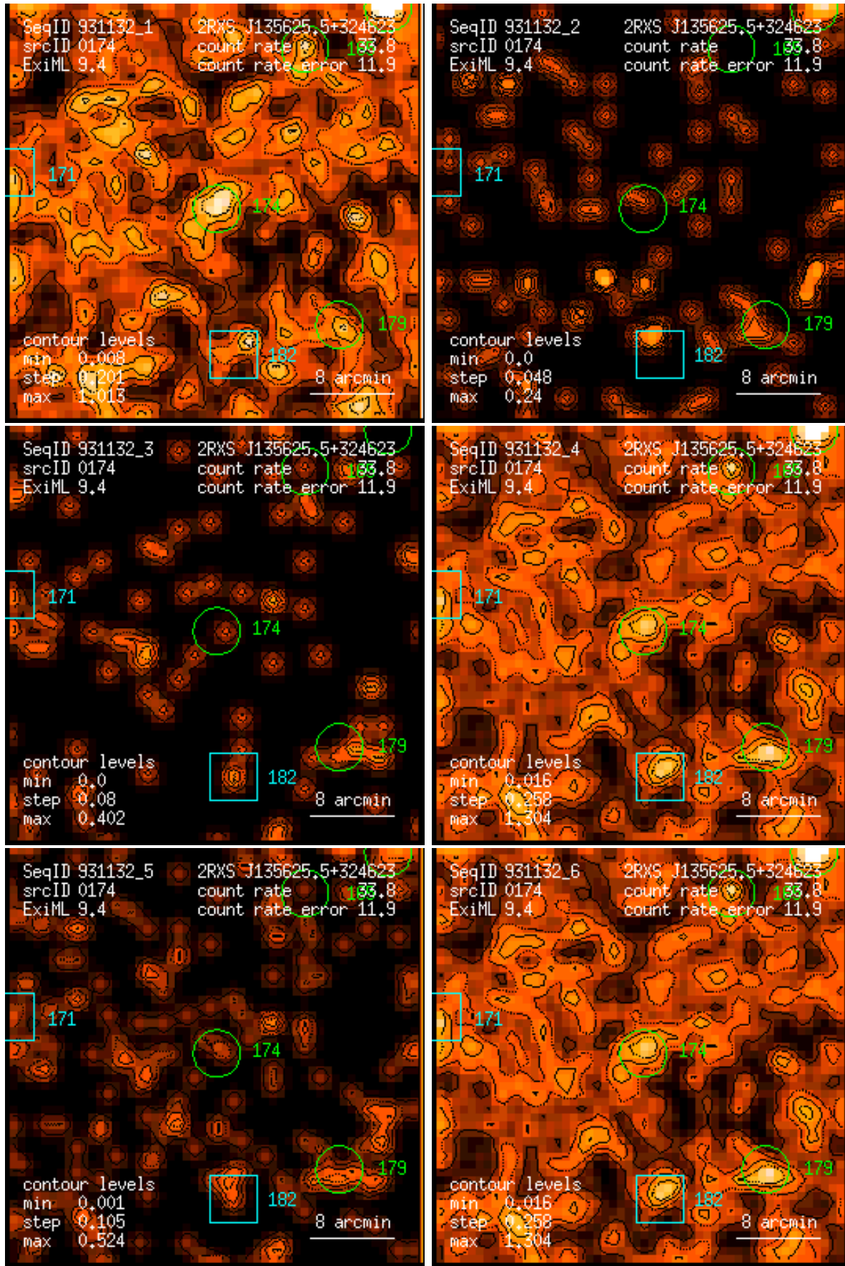
Figure 174: RASS 931132: detection 0174: band rate images, Gaussian filter: (1) PSPC channels 11 – 41, (2) 52 – 90, (3) 91 – 201, (4) 11 – 235, (5) 52 – 201, (6) 11 – 201. Broad band rates in counts/ks. Band rate contour levels in counts/ks/arcmin 2 .
