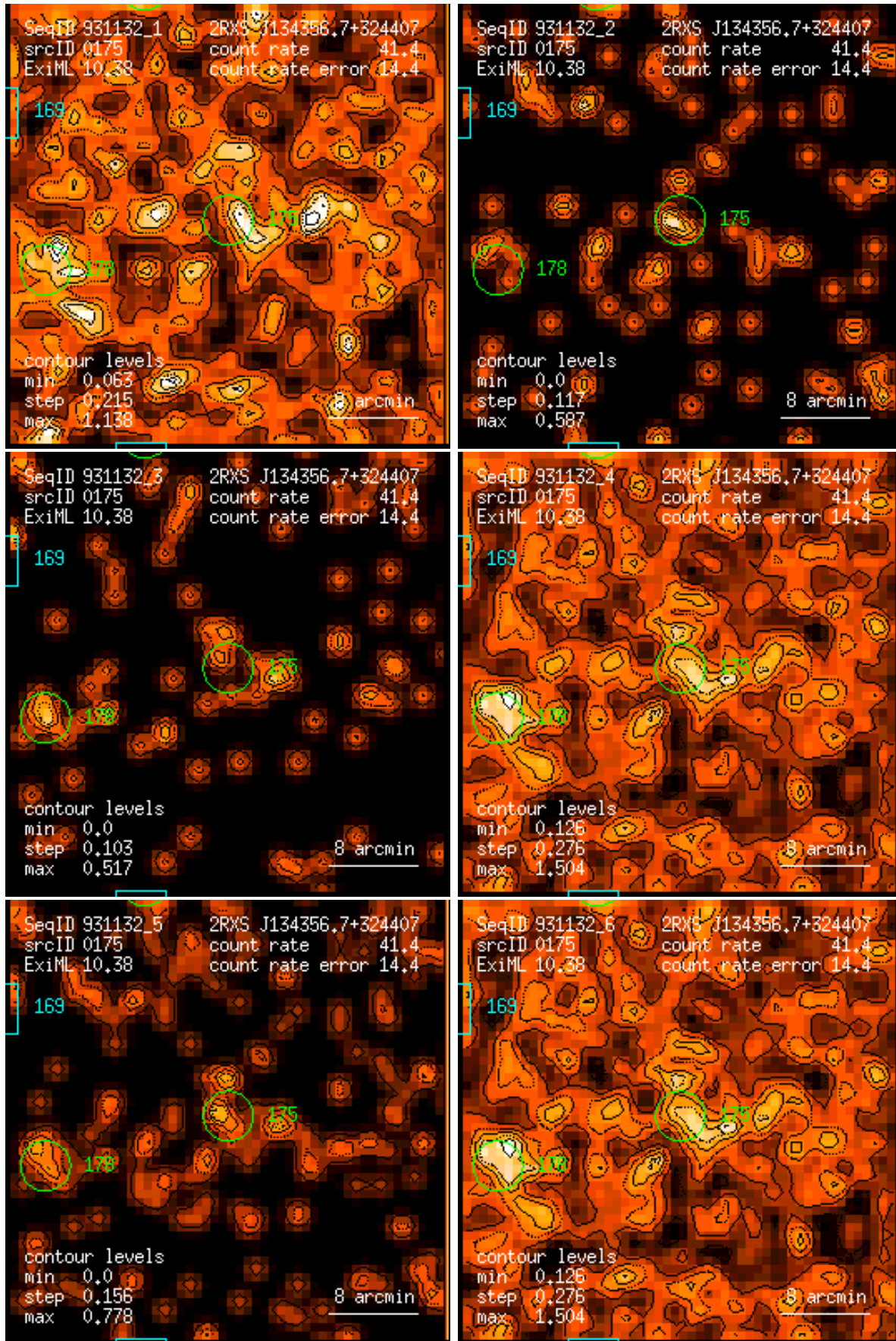
Figure 175: RASS 931132: detection 0175: band rate images, Gaussian filter: (1) PSPC channels 11 – 41, (2) 52 – 90, (3) 91 – 201, (4) 11 – 235, (5) 52 – 201, (6) 11 – 201. Broad band rates in counts/ks. Band rate contour levels in counts/ks/arcmin 2 .
