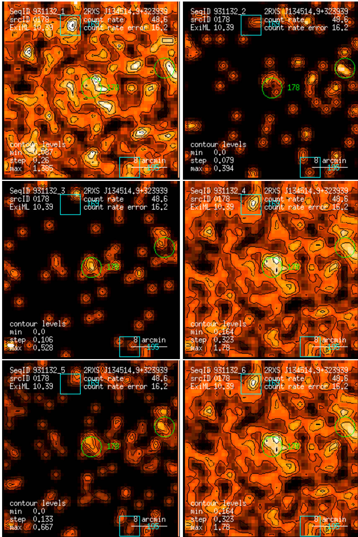
Figure 178: RASS 931132: detection 0178: band rate images, Gaussian filter: (1) PSPC channels 11 – 41, (2) 52 – 90, (3) 91 – 201, (4) 11 – 235, (5) 52 – 201, (6) 11 – 201. Broad band rates in counts/ks. Band rate contour levels in counts/ks/arcmin 2 .
