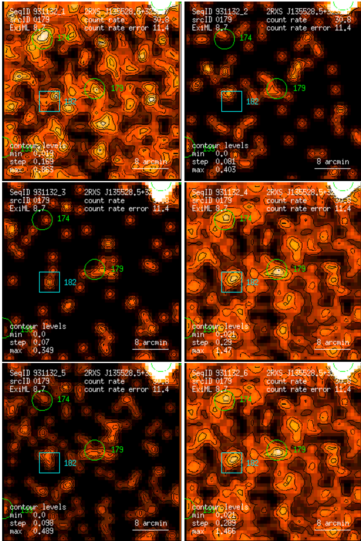
Figure 179: RASS 931132: detection 0179: band rate images, Gaussian filter: (1) PSPC channels 11 – 41, (2) 52 – 90, (3) 91 – 201, (4) 11 – 235, (5) 52 – 201, (6) 11 – 201. Broad band rates in counts/ks. Band rate contour levels in counts/ks/arcmin 2 .
