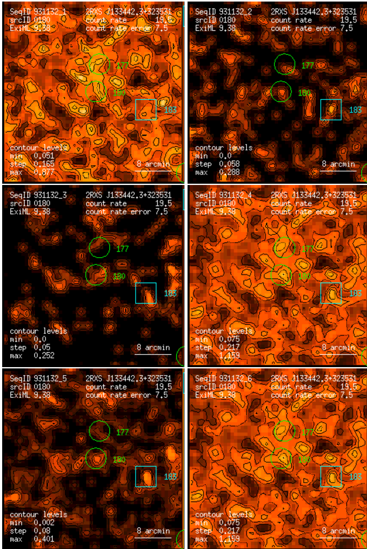
Figure 180: RASS 931132: detection 0180: band rate images, Gaussian filter: (1) PSPC channels 11 – 41, (2) 52 – 90, (3) 91 – 201, (4) 11 – 235, (5) 52 – 201, (6) 11 – 201. Broad band rates in counts/ks. Band rate contour levels in counts/ks/arcmin 2 .
