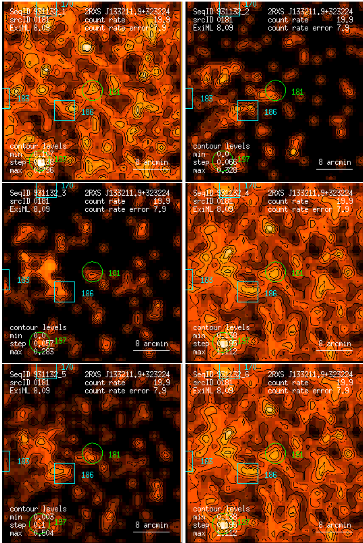
Figure 181: RASS 931132: detection 0181: band rate images, Gaussian filter: (1) PSPC channels 11 – 41, (2) 52 – 90, (3) 91 – 201, (4) 11 – 235, (5) 52 – 201, (6) 11 – 201. Broad band rates in counts/ks. Band rate contour levels in counts/ks/arcmin 2 .
