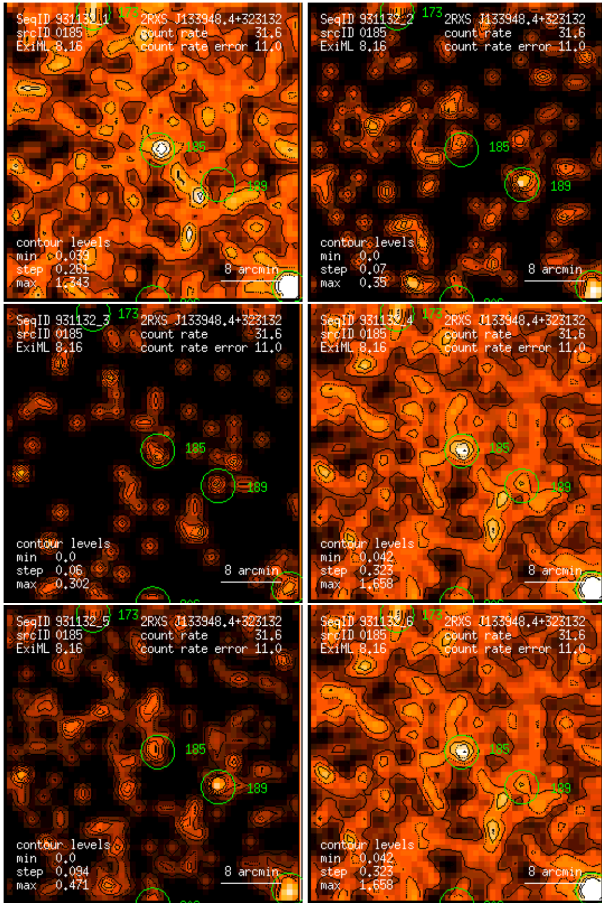
Figure 185: RASS 931132: detection 0185: band rate images, Gaussian filter: (1) PSPC channels 11 – 41, (2) 52 – 90, (3) 91 – 201, (4) 11 – 235, (5) 52 – 201, (6) 11 – 201. Broad band rates in counts/ks. Band rate contour levels in counts/ks/arcmin 2 .
