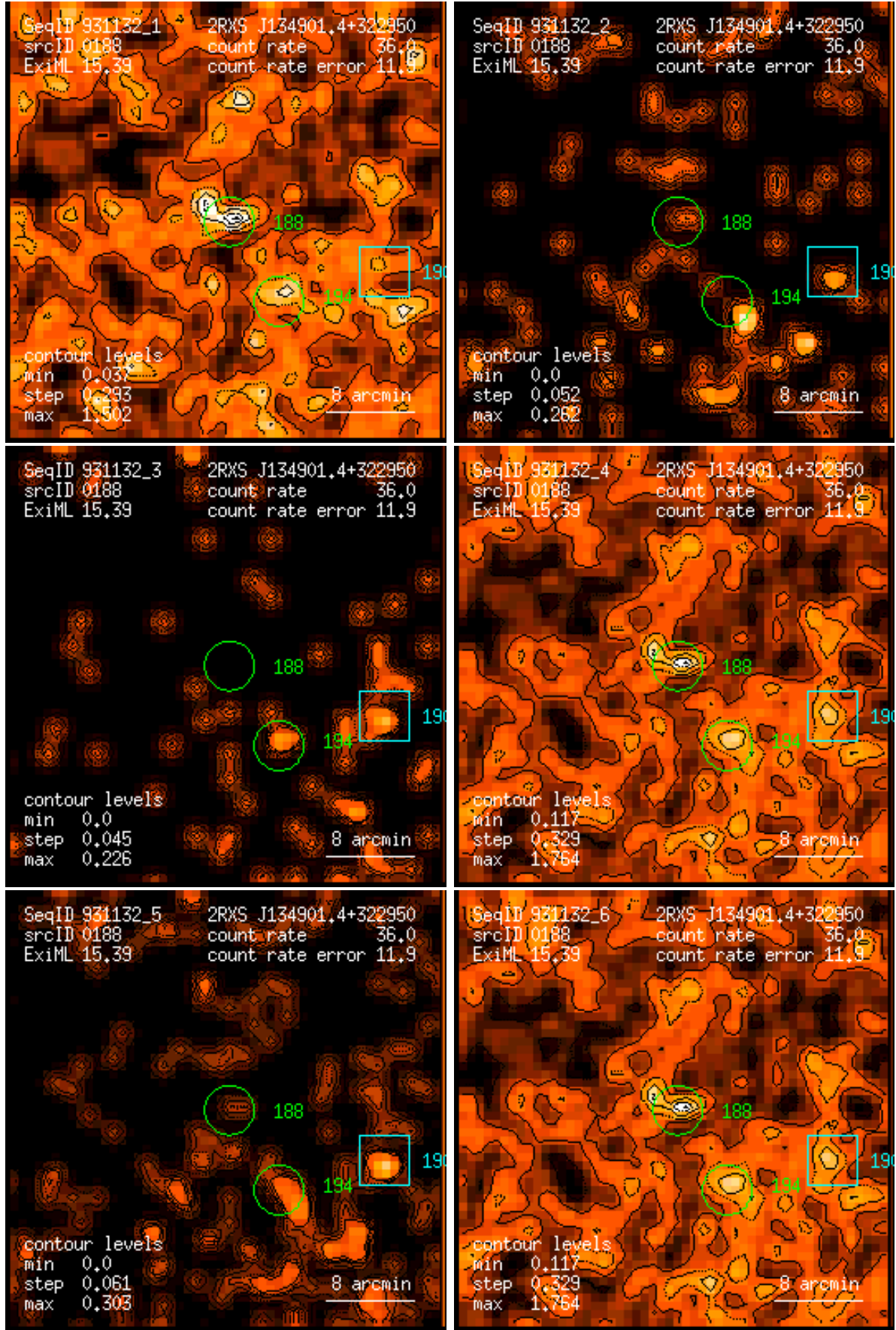
Figure 188: RASS 931132: detection 0188: band rate images, Gaussian filter: (1) PSPC channels 11 – 41, (2) 52 – 90, (3) 91 – 201, (4) 11 – 235, (5) 52 – 201, (6) 11 – 201. Broad band rates in counts/ks. Band rate contour levels in counts/ks/arcmin 2 .
