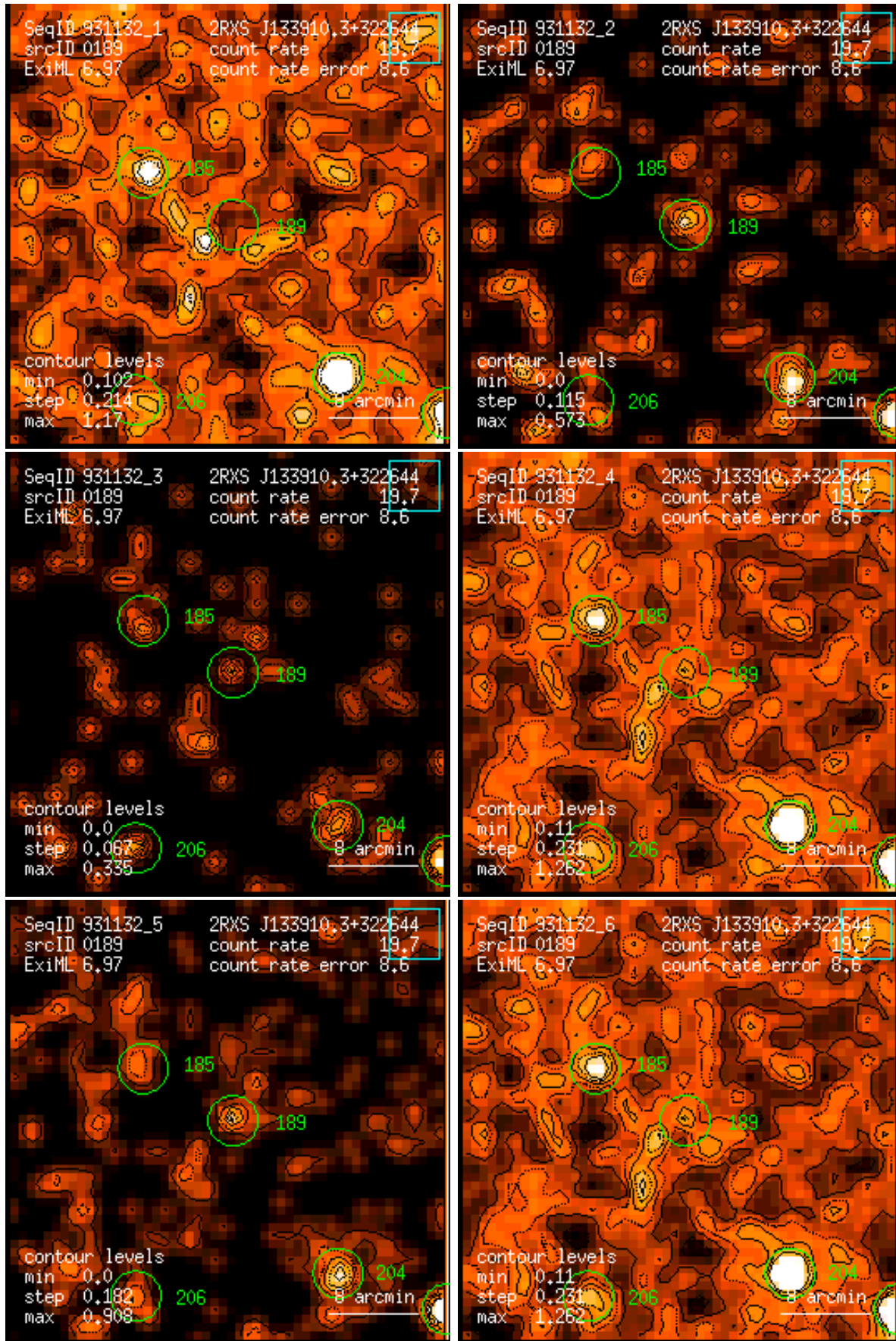
Figure 189: RASS 931132: detection 0189: band rate images, Gaussian filter: (1) PSPC channels 11 – 41, (2) 52 – 90, (3) 91 – 201, (4) 11 – 235, (5) 52 – 201, (6) 11 – 201. Broad band rates in counts/ks. Band rate contour levels in counts/ks/arcmin 2 .
