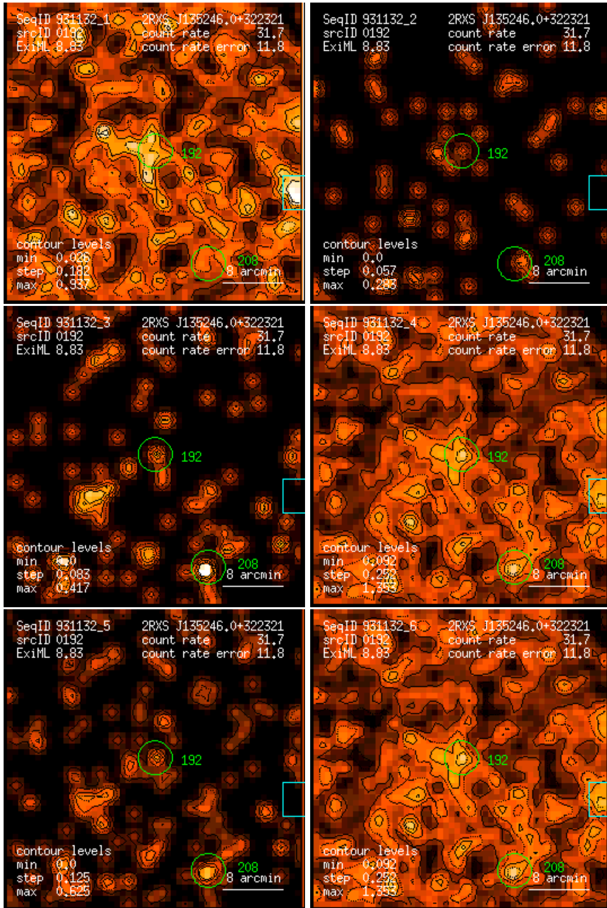
Figure 192: RASS 931132: detection 0192: band rate images, Gaussian filter: (1) PSPC channels 11 – 41, (2) 52 – 90, (3) 91 – 201, (4) 11 – 235, (5) 52 – 201, (6) 11 – 201. Broad band rates in counts/ks. Band rate contour levels in counts/ks/arcmin 2 .
