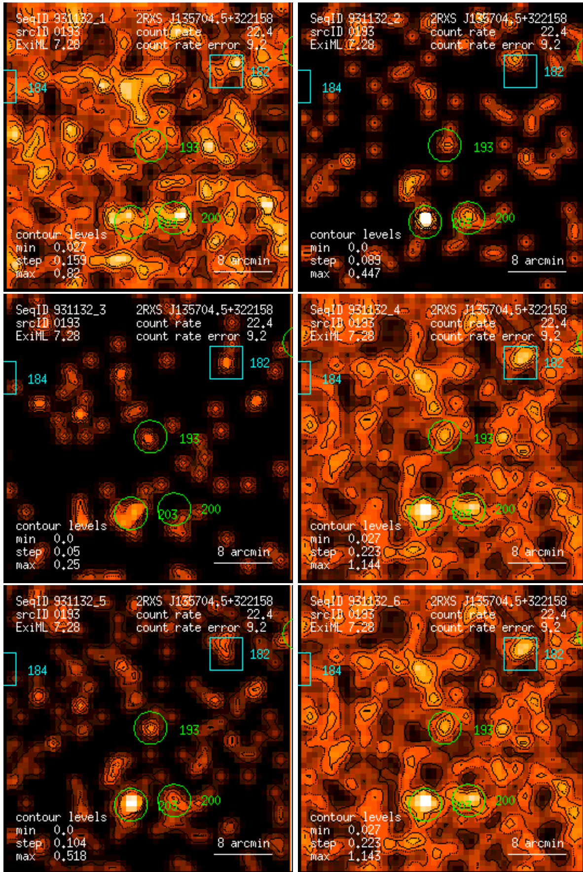
Figure 193: RASS 931132: detection 0193: band rate images, Gaussian filter: (1) PSPC channels 11 – 41, (2) 52 – 90, (3) 91 – 201, (4) 11 – 235, (5) 52 – 201, (6) 11 – 201. Broad band rates in counts/ks. Band rate contour levels in counts/ks/arcmin 2 .
