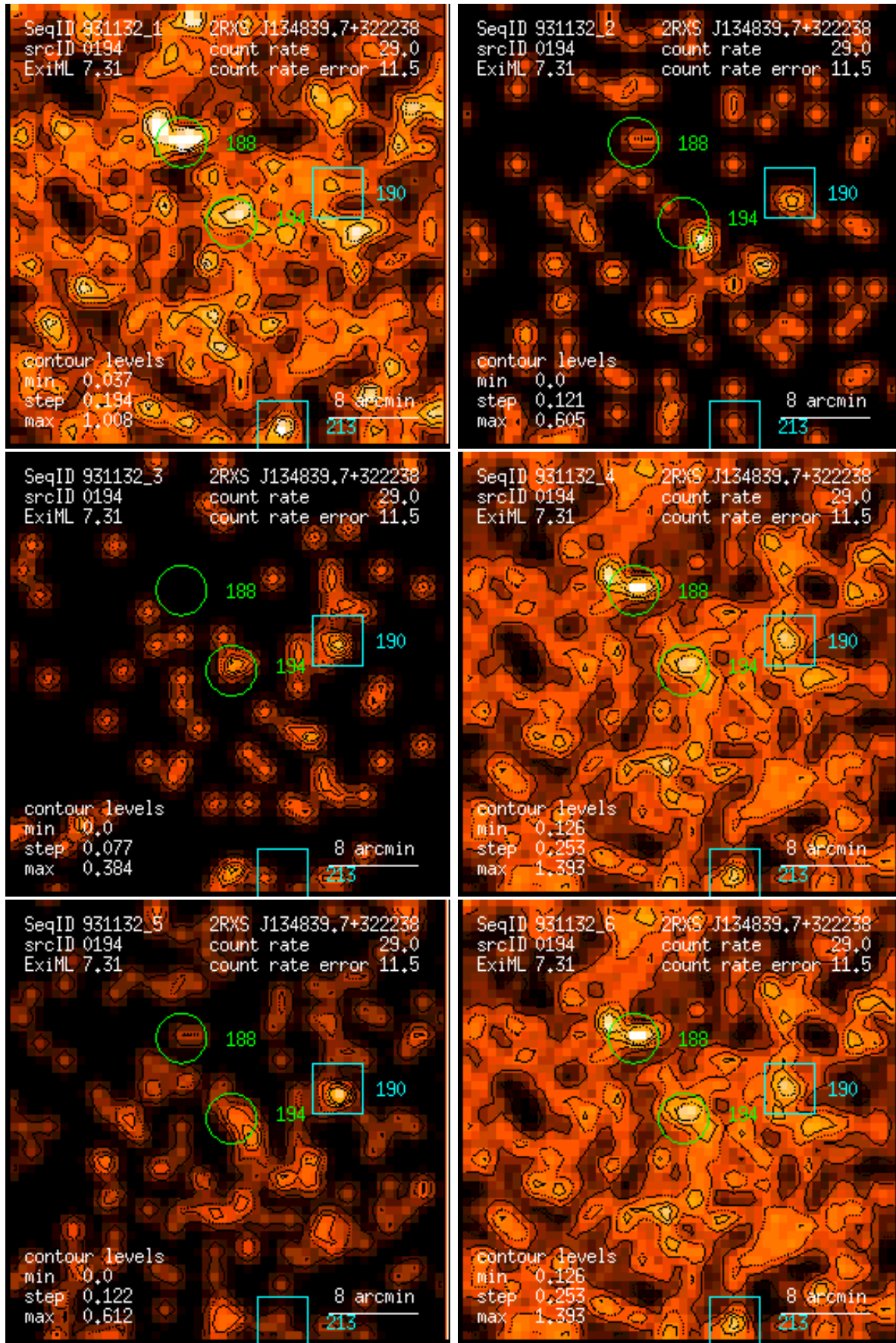
Figure 194: RASS 931132: detection 0194: band rate images, Gaussian filter: (1) PSPC channels 11 – 41, (2) 52 – 90, (3) 91 – 201, (4) 11 – 235, (5) 52 – 201, (6) 11 – 201. Broad band rates in counts/ks. Band rate contour levels in counts/ks/arcmin 2 .
