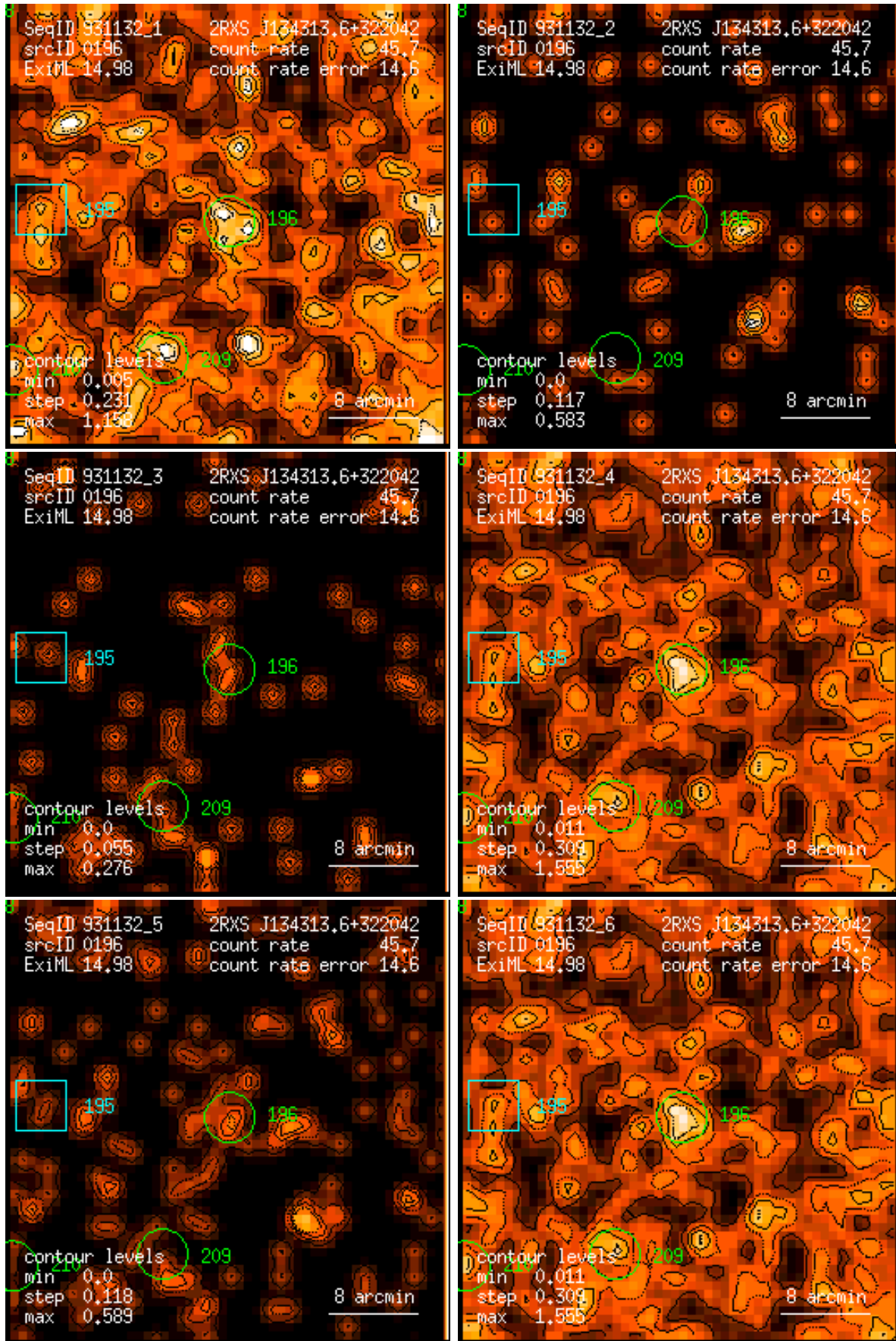
Figure 196: RASS 931132: detection 0196: band rate images, Gaussian filter: (1) PSPC channels 11 – 41, (2) 52 – 90, (3) 91 – 201, (4) 11 – 235, (5) 52 – 201, (6) 11 – 201. Broad band rates in counts/ks. Band rate contour levels in counts/ks/arcmin 2 .
