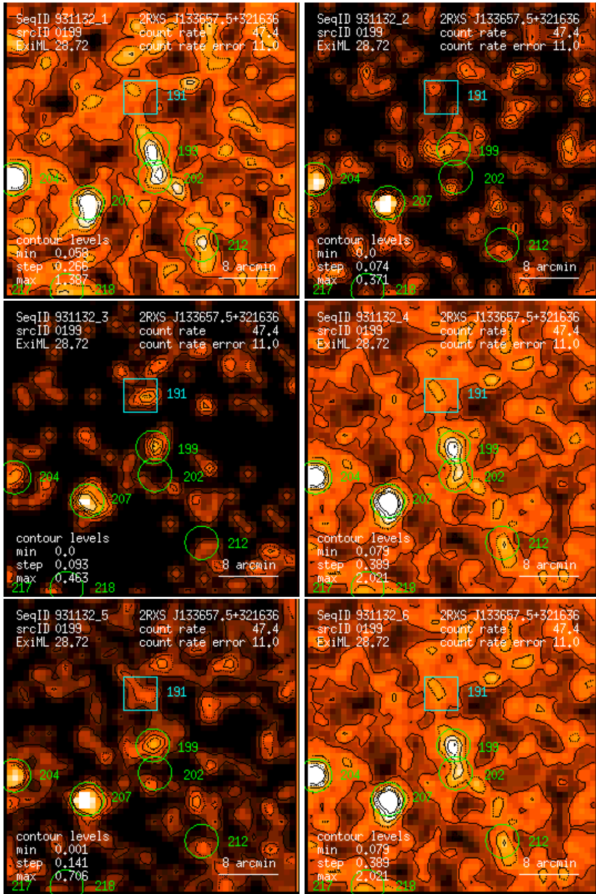
Figure 199: RASS 931132: detection 0199: band rate images, Gaussian filter: (1) PSPC channels 11 – 41, (2) 52 – 90, (3) 91 – 201, (4) 11 – 235, (5) 52 – 201, (6) 11 – 201. Broad band rates in counts/ks. Band rate contour levels in counts/ks/arcmin 2 .
